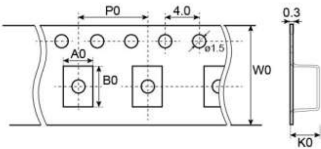
Figure 12 - Tape drawing
