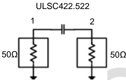
Schematic of 22nF ULSC in transmission mode
