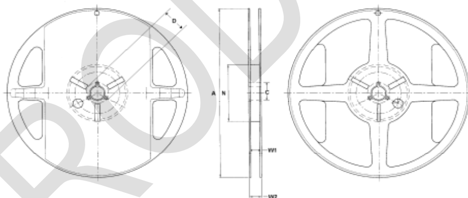
Figure 11 - Reel drawing
