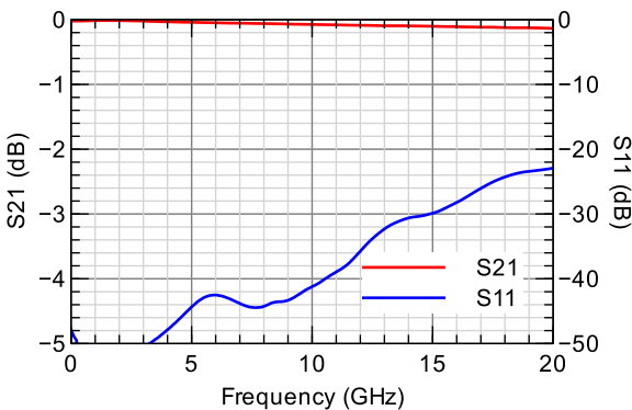
Figure 2 - 22nF ULSC measurement results (module of S-parameters)
