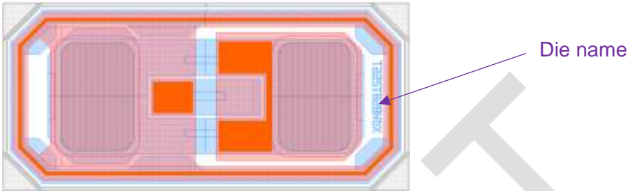
Figure 8 – Layout view
