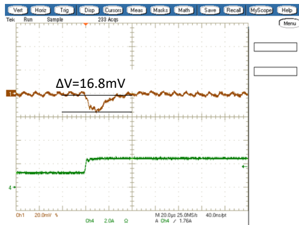
Step Load Transient Response (Vin=5V, Vout1=1.2V, Iout=1.25A to 2.5A) Trace 1=Vout1, 20 mV/div, Trace 4=Iout1, 2.0A/div.
