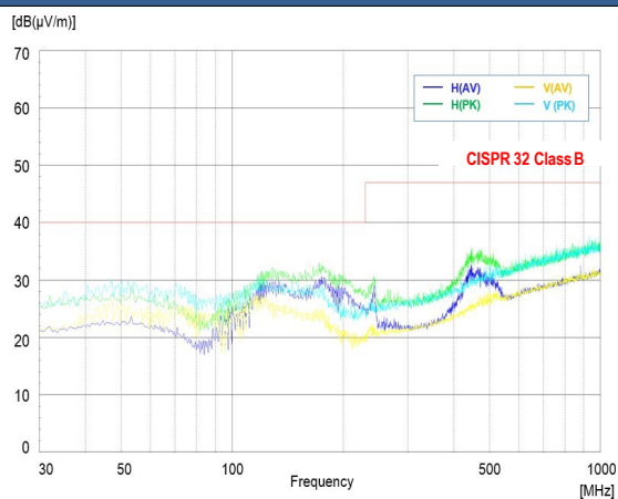
( V_{IN} = 48V , I_{OUT} = 4.25A , T_a = 25degC ) with External Input Filter Figure 10. Radiation Noise
