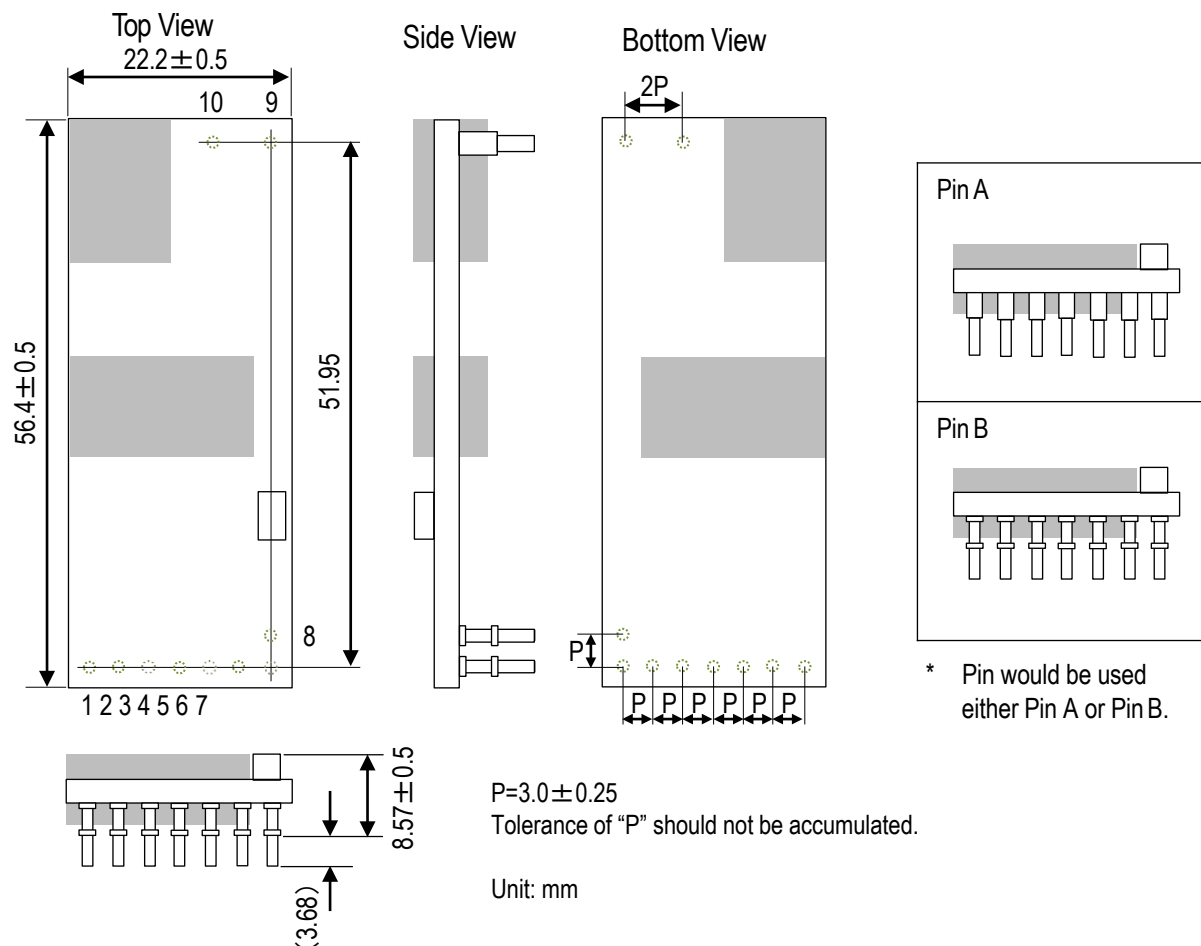
Figure 21. Product Dimensions
