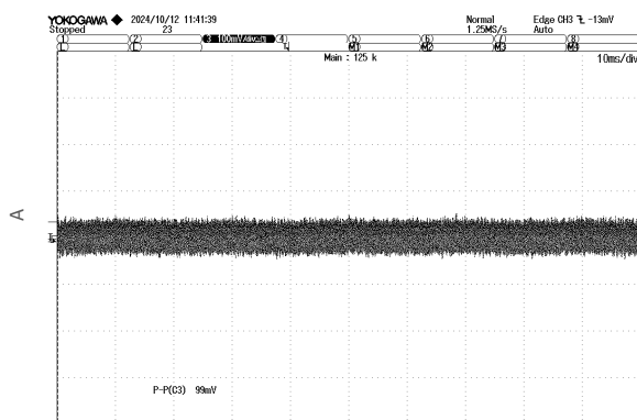
Figure 11. Ripple & Noise 48Vin, Full Load, 1µF+10µF
