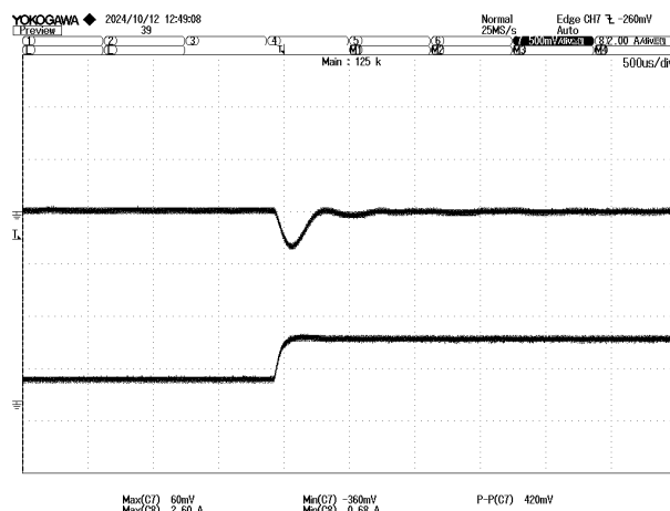
Figure 10. Output Transient Response 48Vin, 25%-75% Load2
