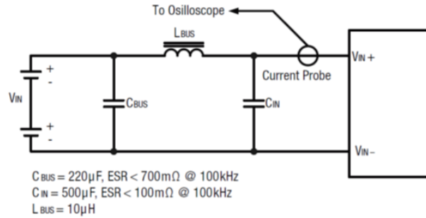
Figure 23. Measuring Input Ripple Current
