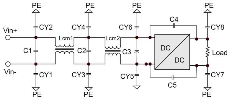
Figure 24. Recommended Input Filter
