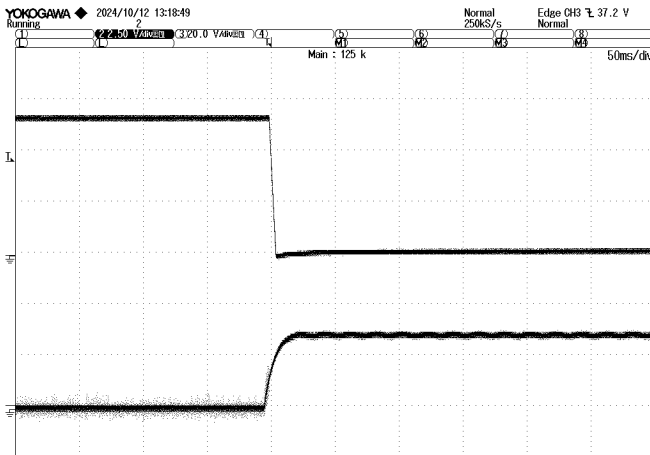
Figure 3. Enable OFF 48Vin, Full Load, 270μF min. cap load
