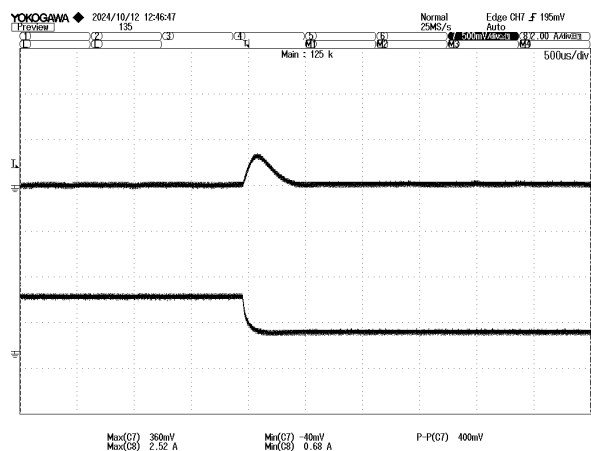
Figure 9. Output Transient Response 48Vin, 25%-75% Load
