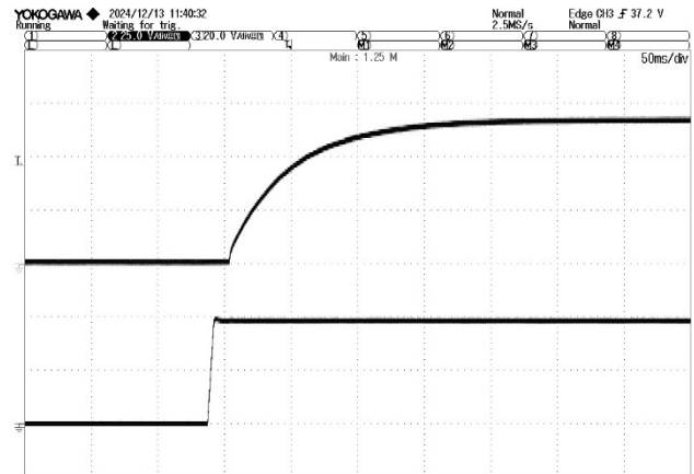
Figure 2. Vin ON 48Vin, Full Load, 270μF min. cap load
