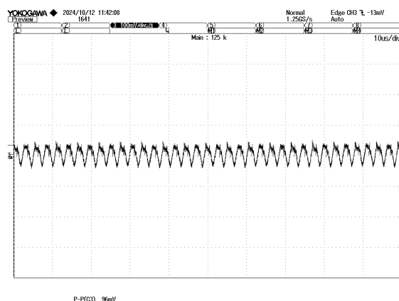
Figure 12. Ripple & Noise 48Vin, Full Load, 1µF+10µF
