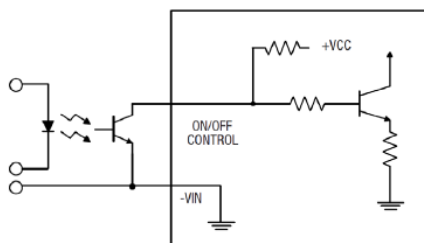
Figure 26. Driving the On/Off Control Pin (suggested circuit)
