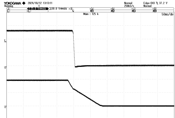
Figure 4. Vin OFF 48Vin, Full Load, 270μF min. cap load
