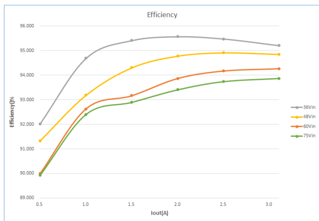
Figure 7. Efficiency Vs. Line Voltage & Load Current @ 25°C
