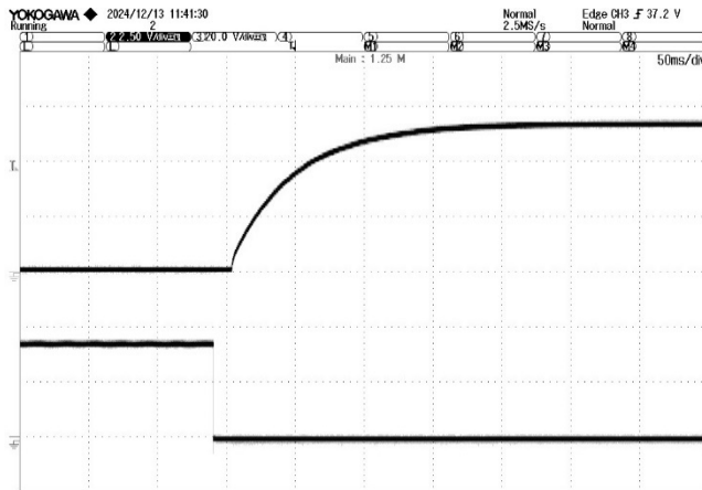
Figure 1. Enable ON 48Vin, Full Load, 270μF min. cap load
