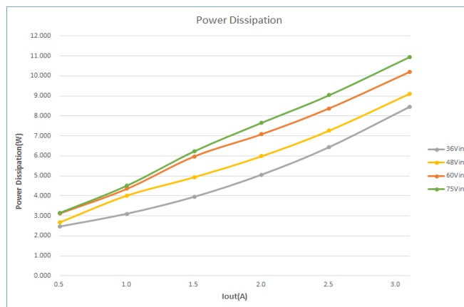
Figure 8. Power Dissipation vs. Load Current @ 25°C
