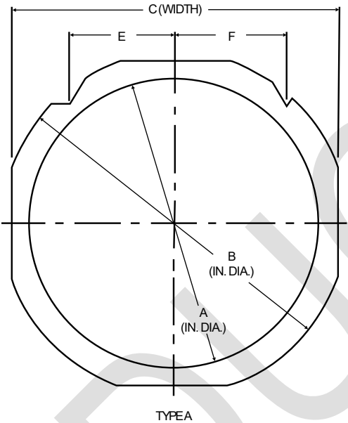
Figure 8 – Film frame drawing
