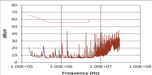
NXJ1S0505(P)T(6)MC (Quasi-Peak)
