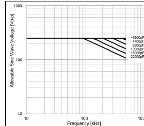
Chip(L×W): 3.2×1.6mm C0G(5C) Char. Rated Voltage:DC250V
