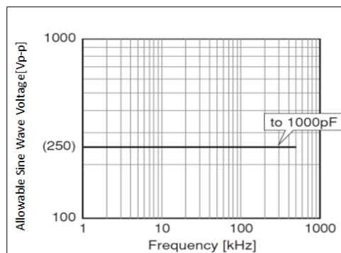
Chip(L×W): 1.0×0.5mm 1.6×0.8mm C0G(5C) Char. Rated Voltage:DC250V
