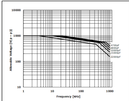
Chip(L×W): 3.2×2.5mm C0G(5C) Char. Rated Voltage : DC1kV
