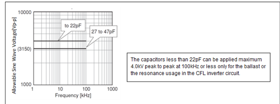
Chip(L×W): 4.5×2.0mm C0G(5C) Char. Rated Voltage:DC3.15kV
