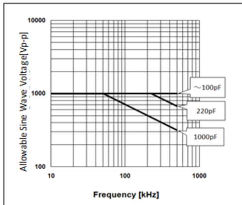
Chip(L×W): 3.2×1.6mm C0G(5C) Char. Rated Voltage:DC1kV
