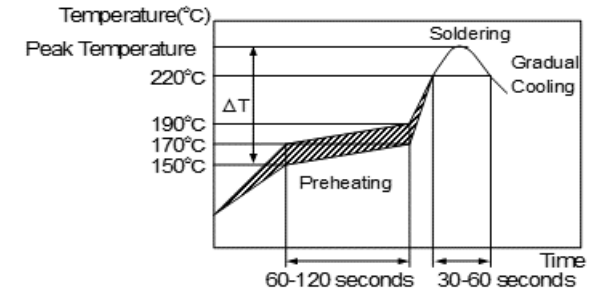
[ Allowable Reflow Soldering Temperature and Time ]
