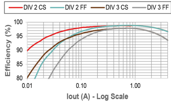
Figure 1. Typical efficiency with V_{IN}=7.7V in divide-by-2 and V_{IN}=11.55V in divide-by-3, fixed frequency (FF) and cycle skip (CS) modes
