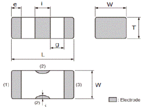
image:Dimension
