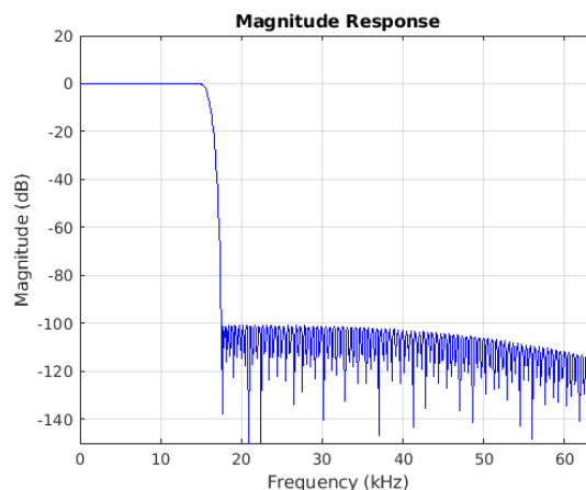
Figure 7-2. Stopband Magnitude
