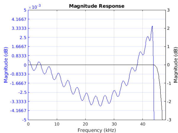
Figure 7-19. Passband Magnitude
