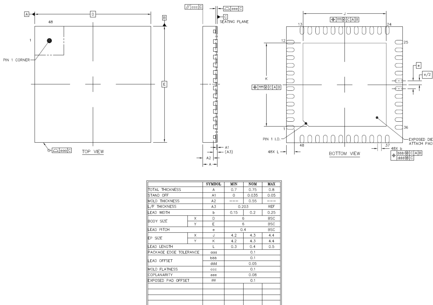
Figure 9-1. QFN Package Drawing
