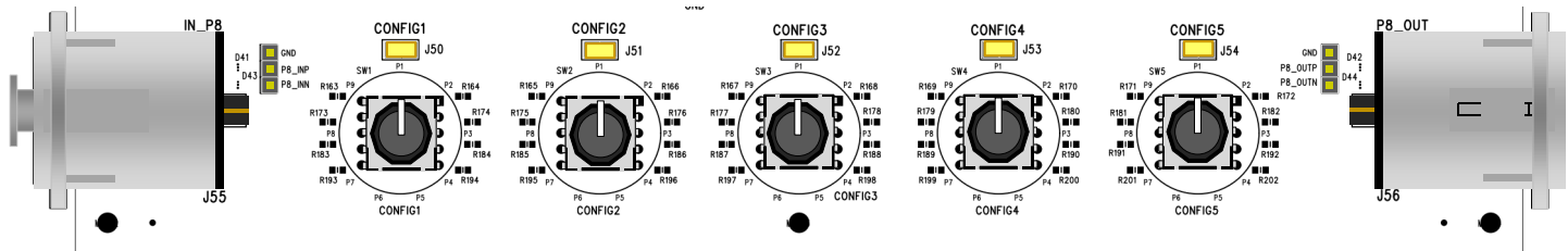
Figure 13: Dungalass Rotary Switches for Hardware Control Mode
