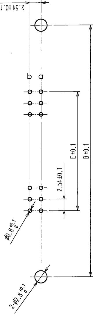
RECOMMENDED P.C.B. HOLE PATTERN(t=1.6±0.1)
