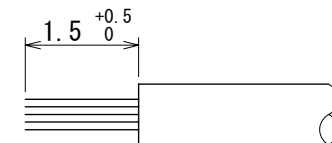
3 Fig.1 Recommended cable preparation dimensions
