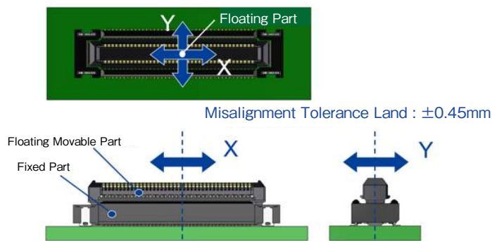
[FX25 Series Header Side : Floating Design]
