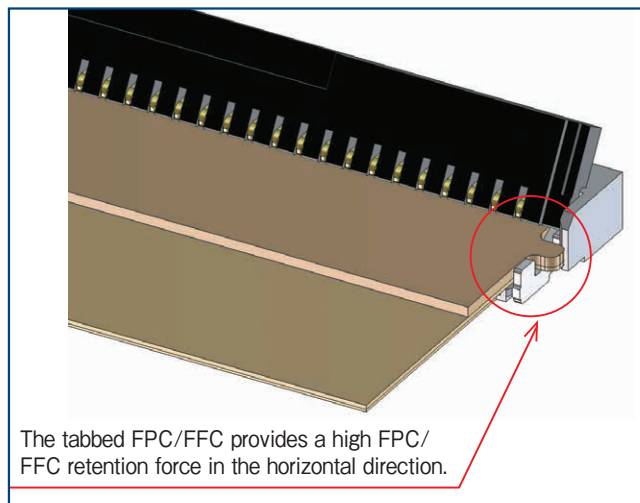
Connection using the FPC/FFC temporary holding mechanism
