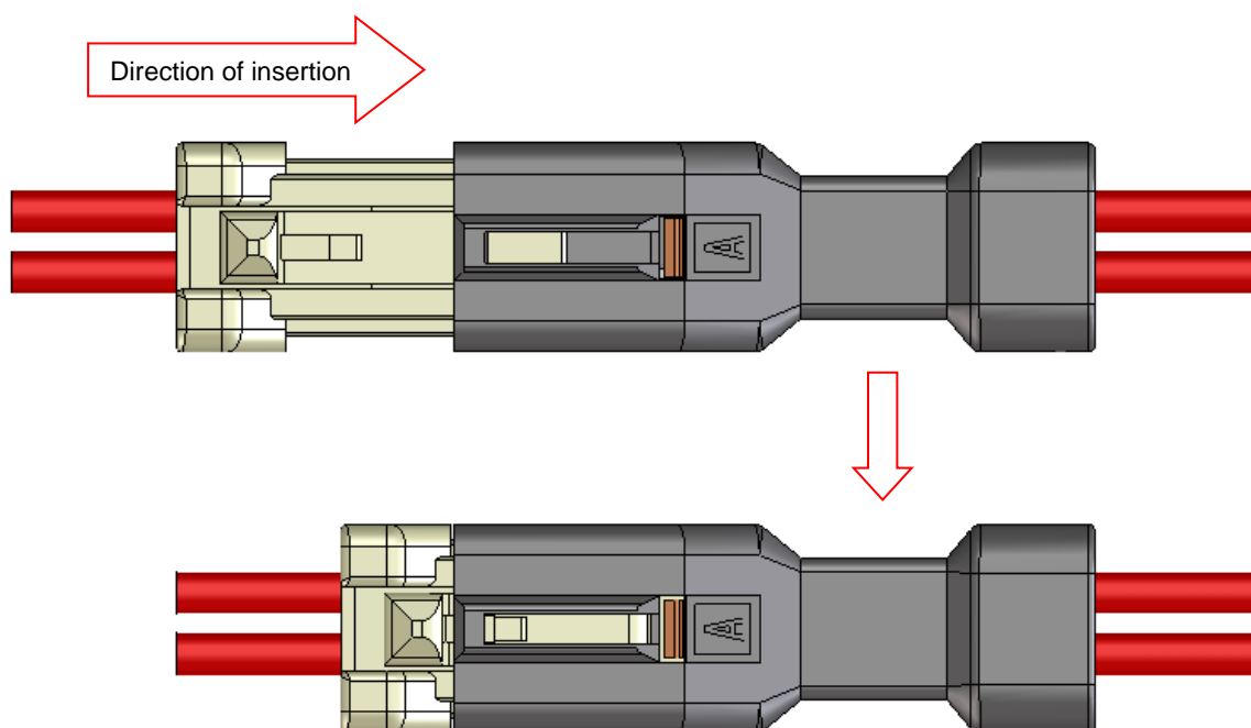
Fig.4 Insertion
