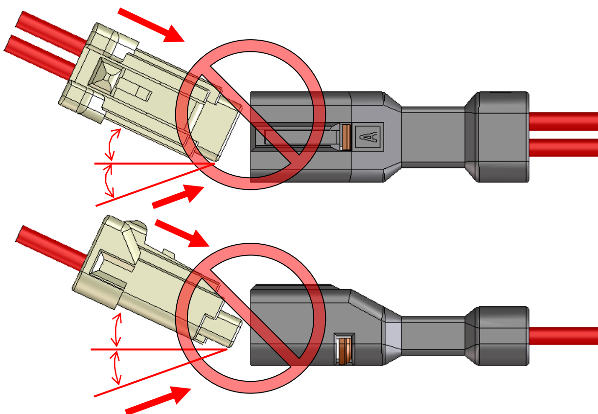
Fig.5 Prohibited insertion
