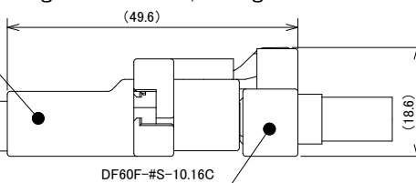
DF60F Finger Protection, Straight Socket
