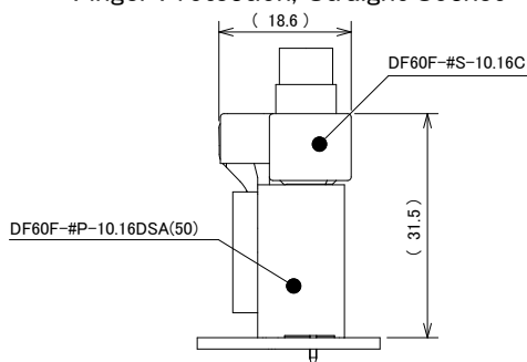
DF60F Finger Protection, Straight Socket
