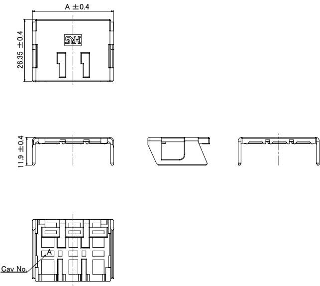
Guide Key: Common for Standard and Another Key Shape (2pos.)
