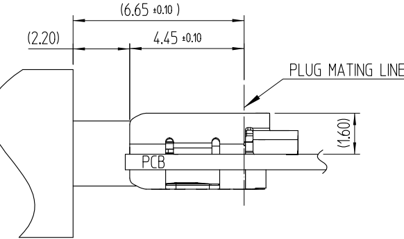
MATED CONDITION (REFERENCE ONLY)
