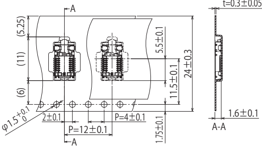
Emboss Carrier Tape Dimensions
