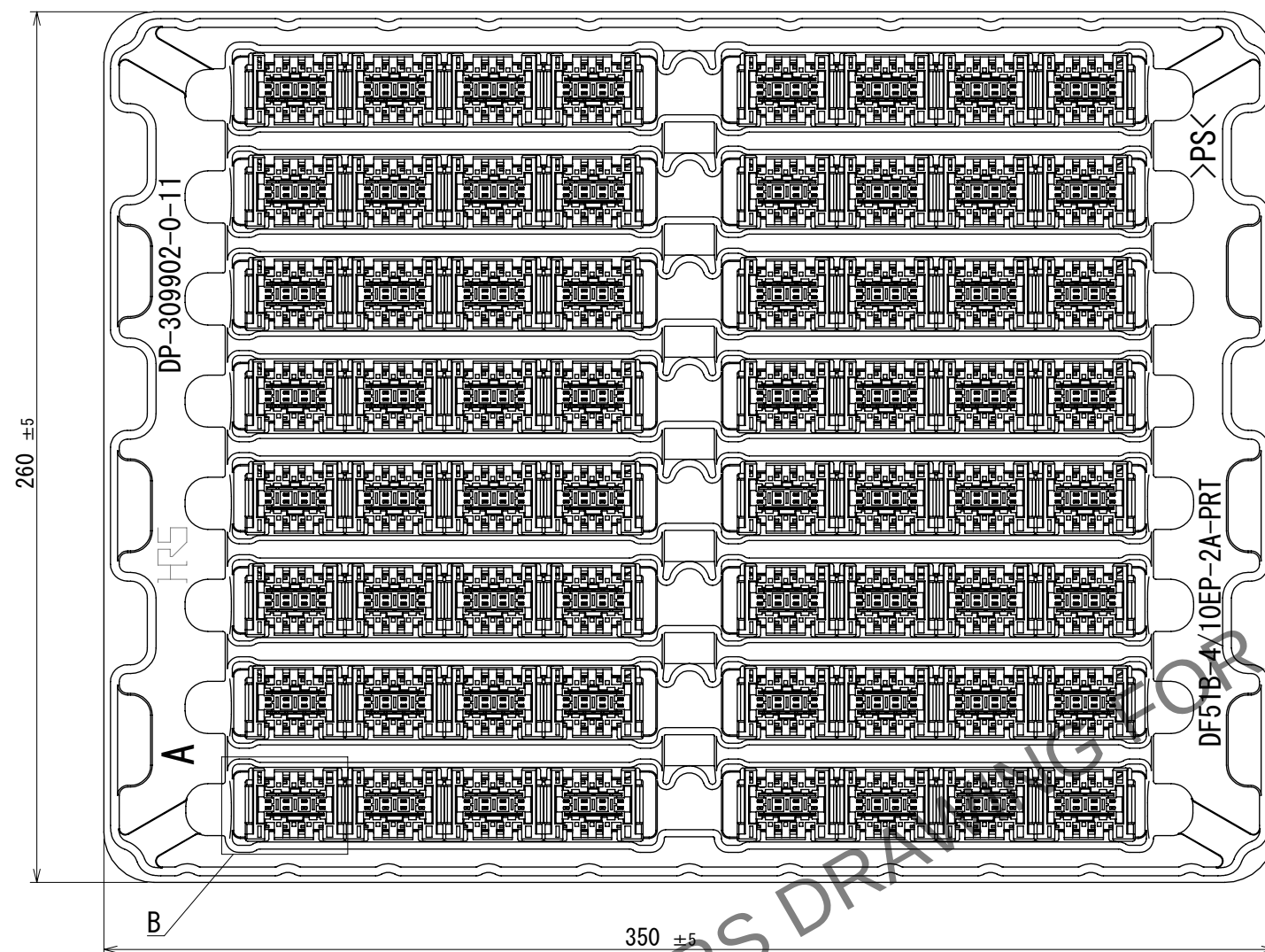
Packing diagram
