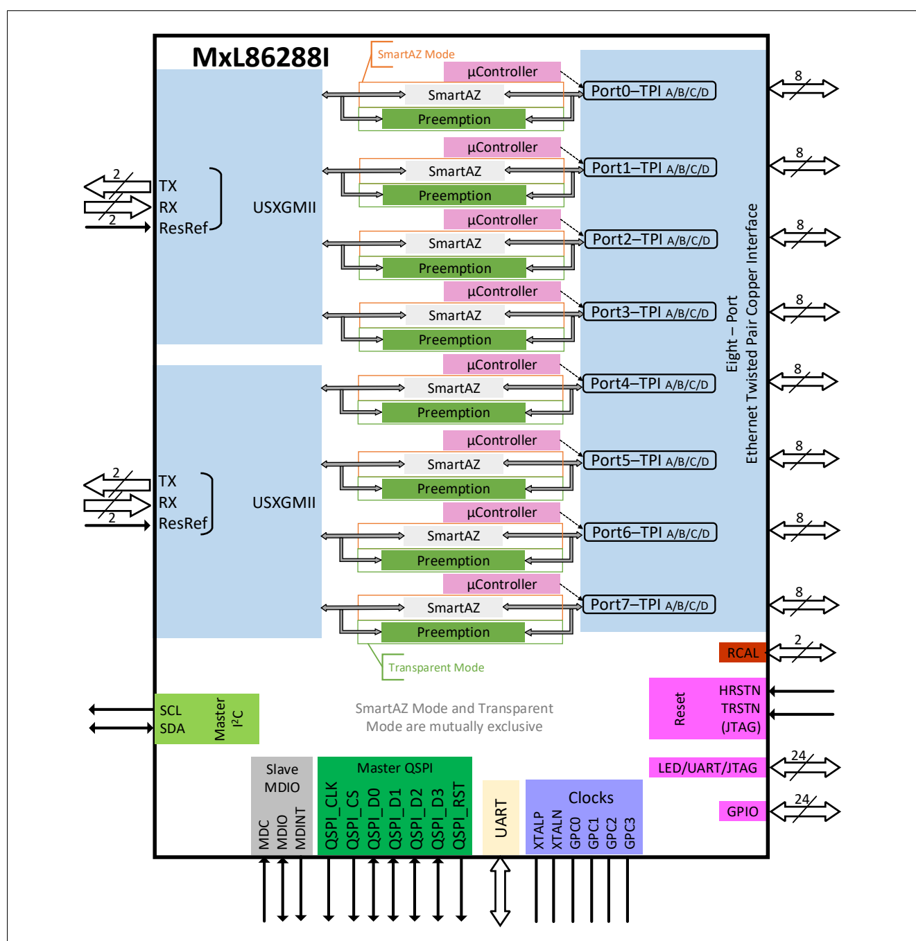
Figure 1 MxL86288I Block Diagram
