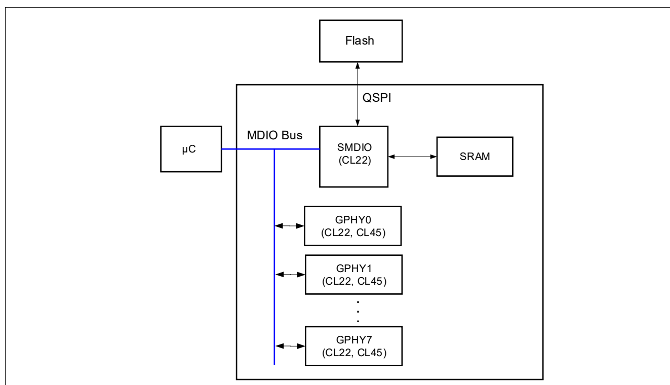
Figure 4 MDIO Slave
