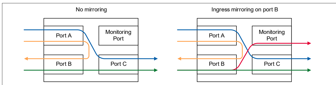
Figure 20 Port Mirroring Examples – Ingress Monitoring
