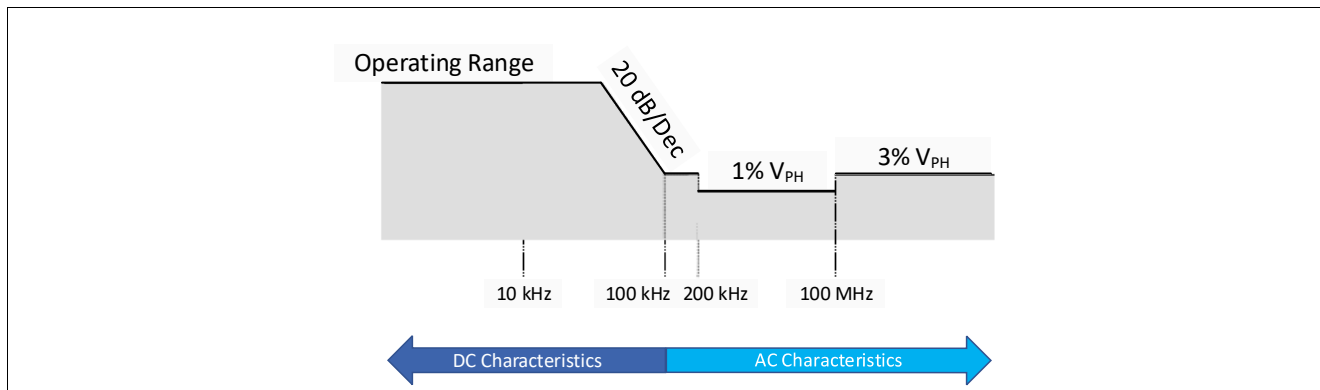
Figure 27 DC and AC Characteristics for V_{PH} Supply
