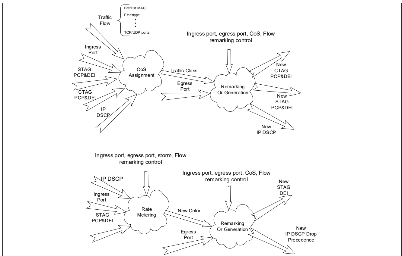
Figure 19 PCP/DSCP/DEI Remarking
