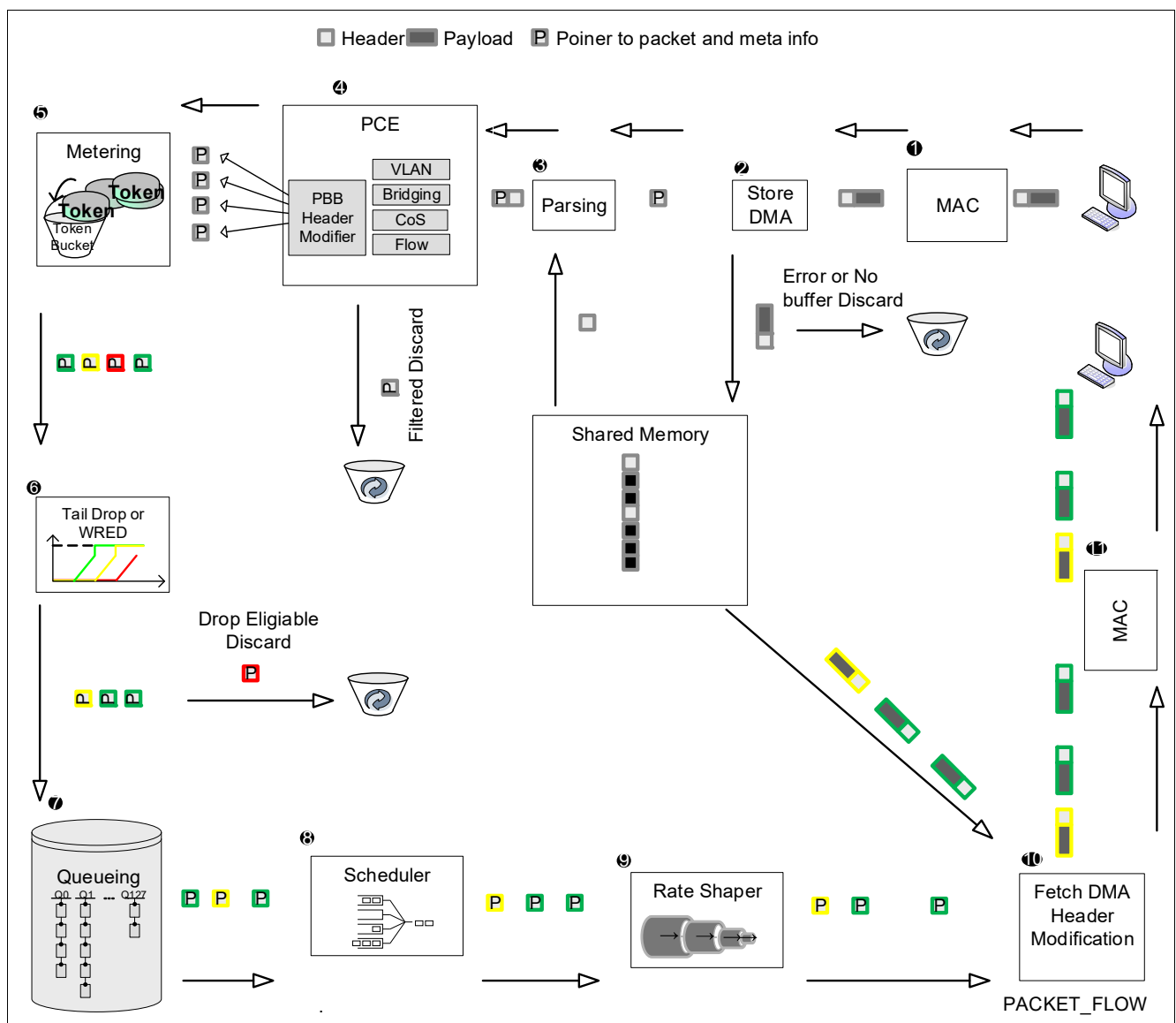
Figure 17 Packet Flow Diagram
