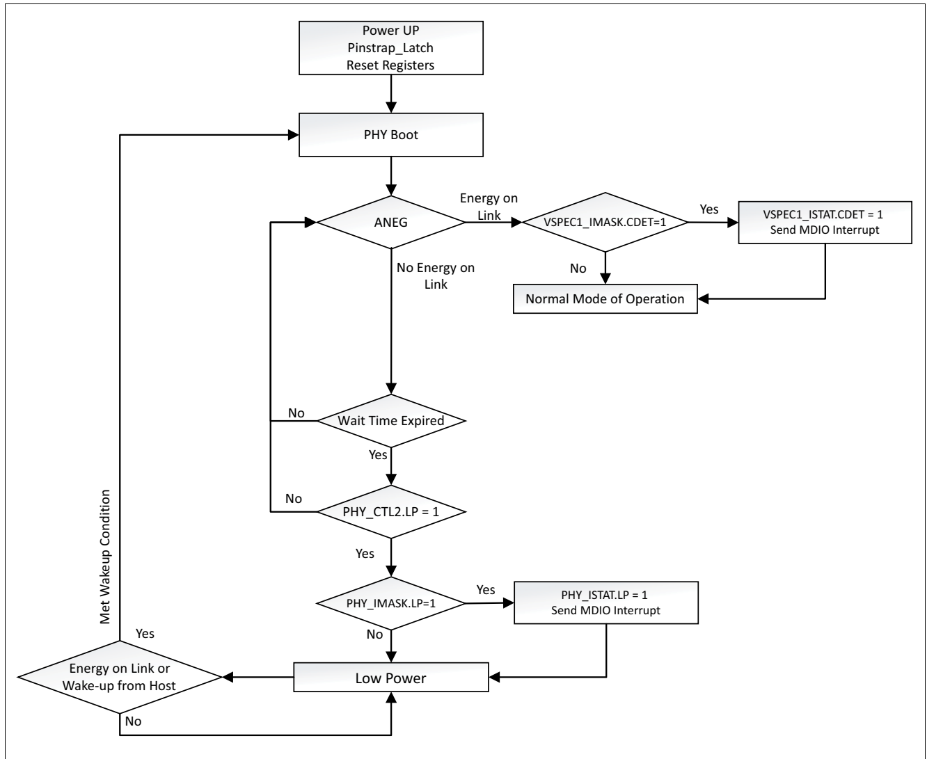
Figure 17 Low Power Sequence
