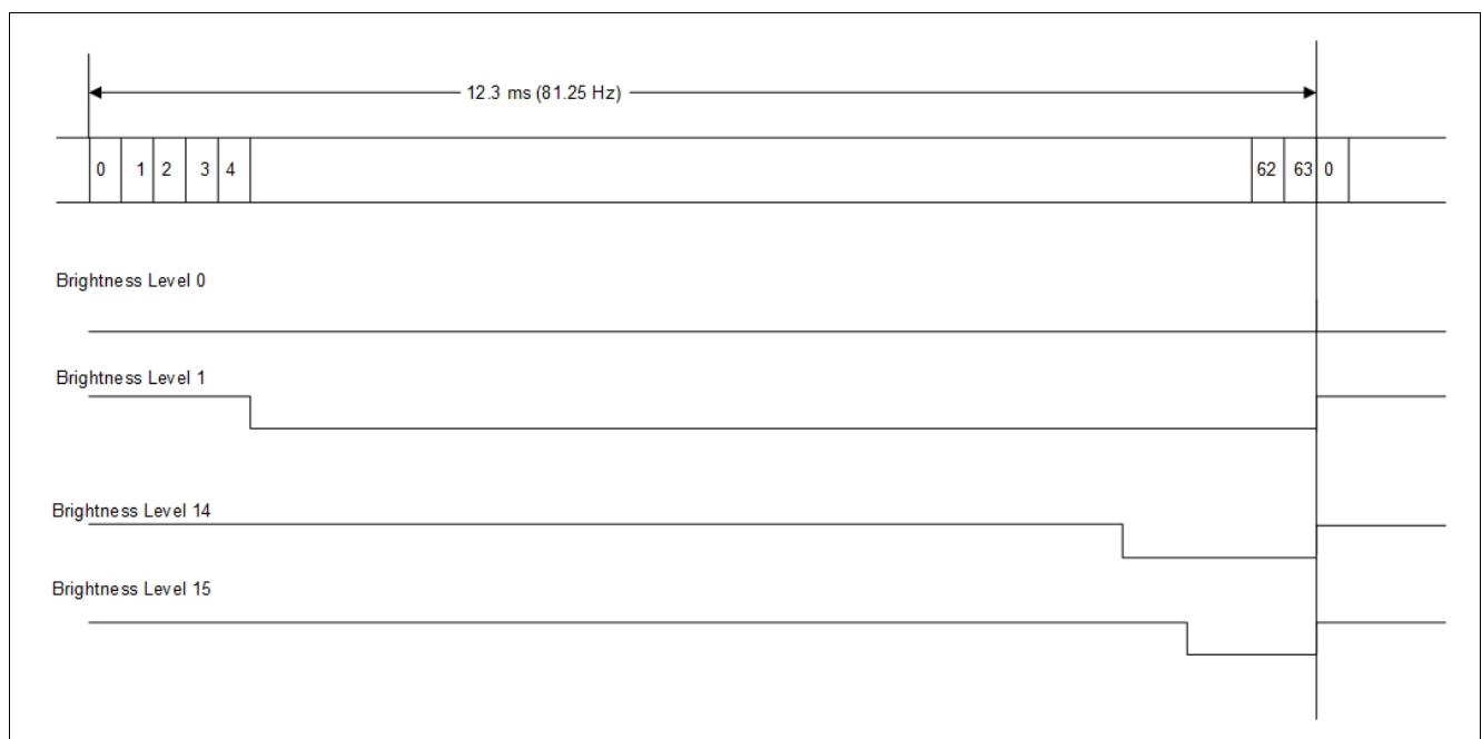
Figure 15 LED Brightness Control by Controlling LED Output Enable/Disable
