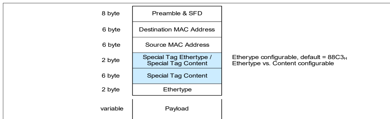
Figure 25 Special Tag Location in the Frame
