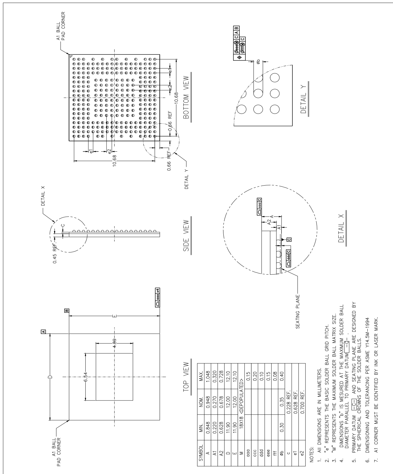
Figure 37 PG-FCLBGA-277 12 mm x 12 mm Package Outline
