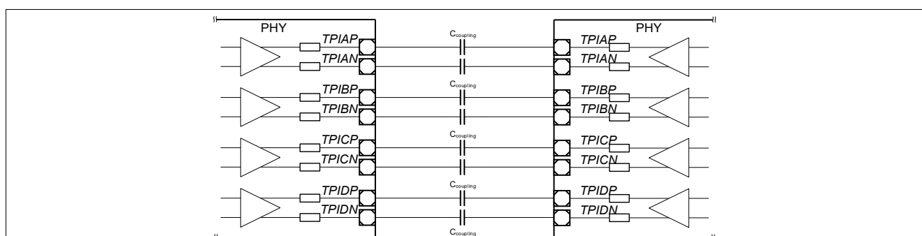
Figure 9 External Circuitry for the Transformerless Ethernet Application
