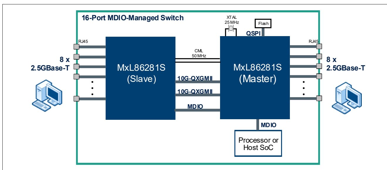
Figure 2 A MDIO-managed 16-port Switch Application
