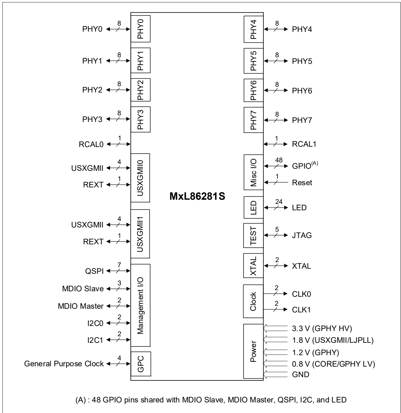
Figure 4 MxL86281S External Signal Overview
