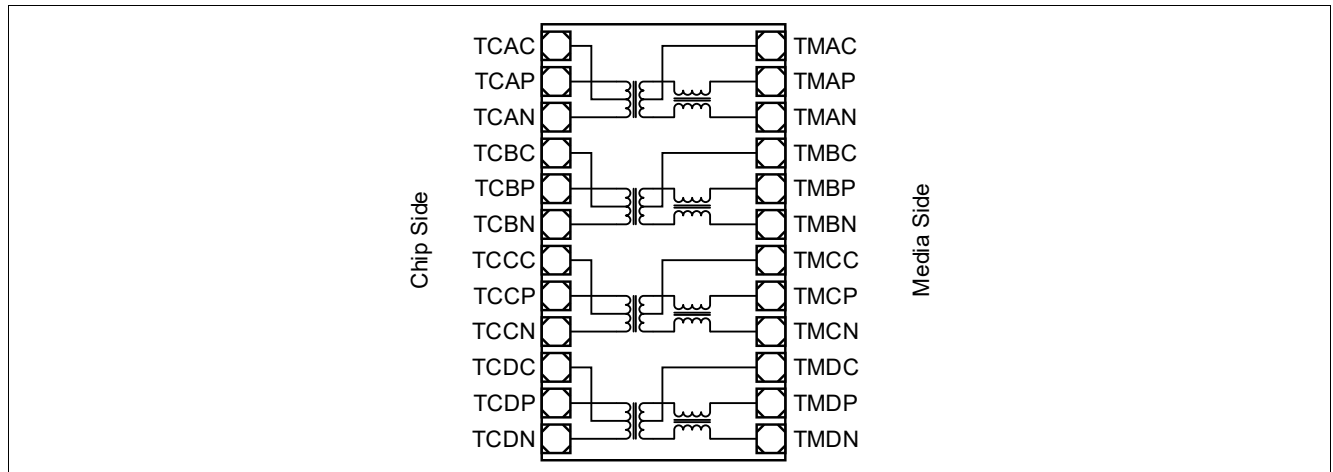
Figure 36 Schematic of an Ethernet Transformer Device
