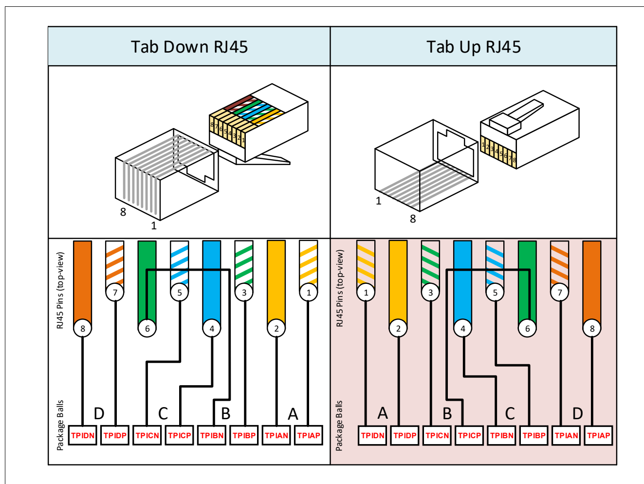
Figure 10 RJ45 Tab Up or Tab Down Configuration
