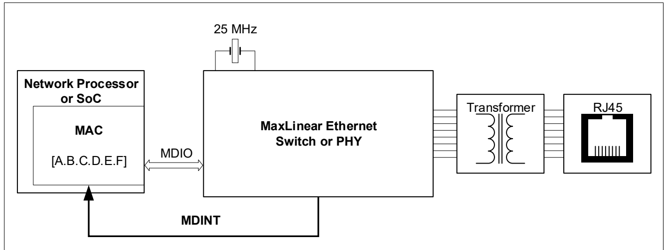
Figure 11 WoL Application Block Diagram
