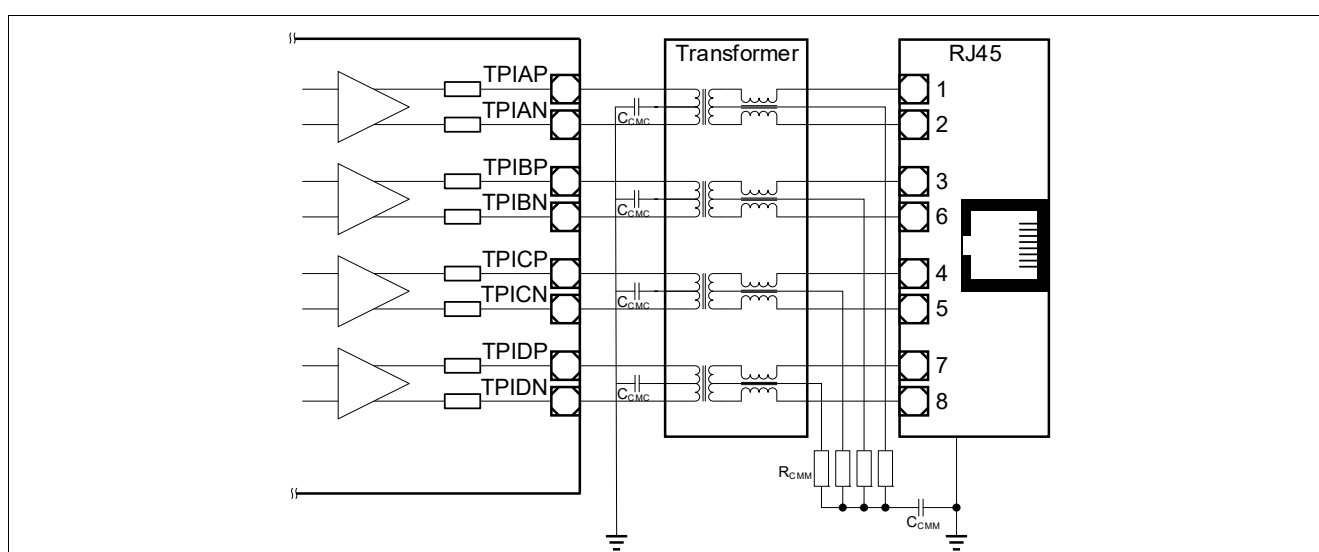
Figure 8 Twisted-Pair Interface of MxL86281S Including Transformer and RJ45 Plug
