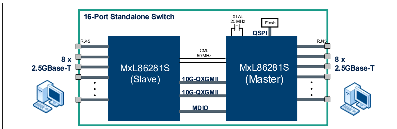
Figure 1 A Standalone 16-port Switch Application
