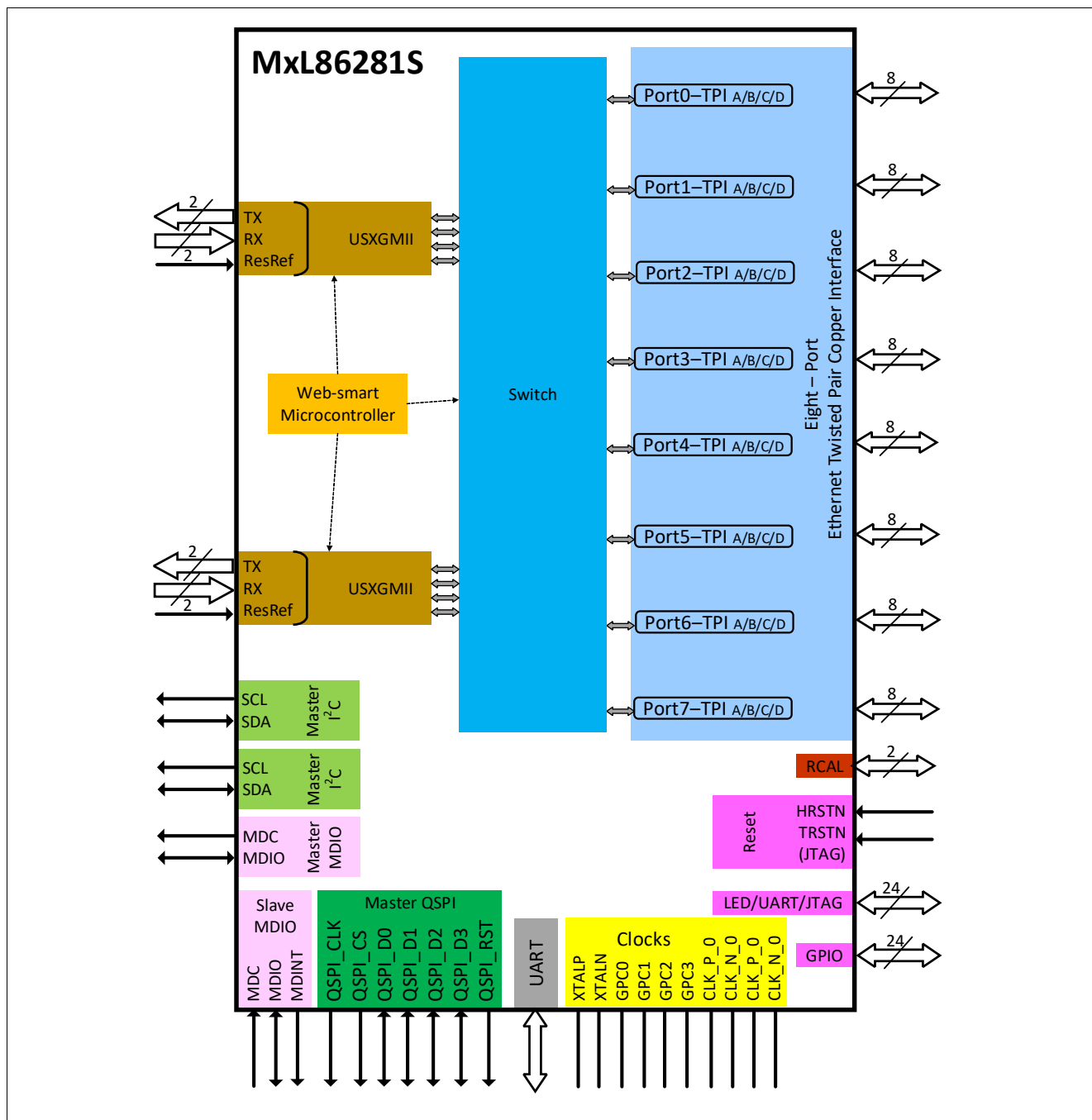
Figure 3 MxL86281S Block Diagram
