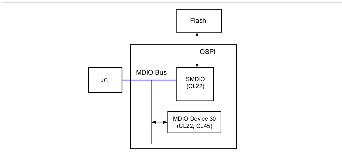
Figure 6 MDIO Slave
