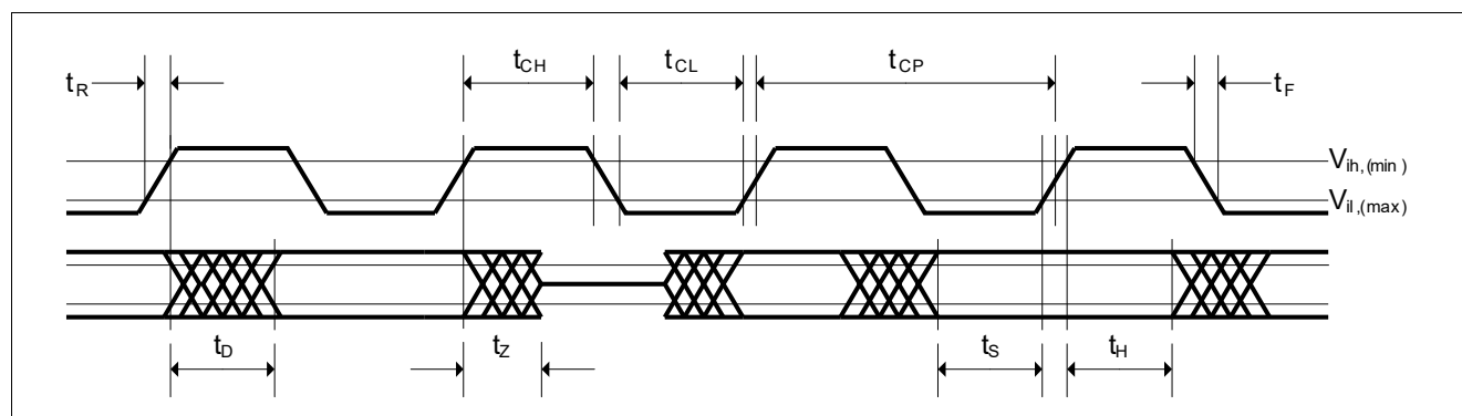
Figure 31 Timing Diagram for the MDIO Master Interface
