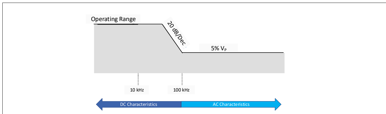
Figure 28 DC and AC Characteristics for V_P Supply
