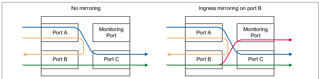
Figure 22 Port Mirroring Examples – Ingress Monitoring
