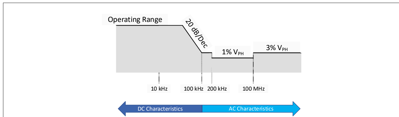
Figure 29 DC and AC Characteristics for V_{PH} Supply
