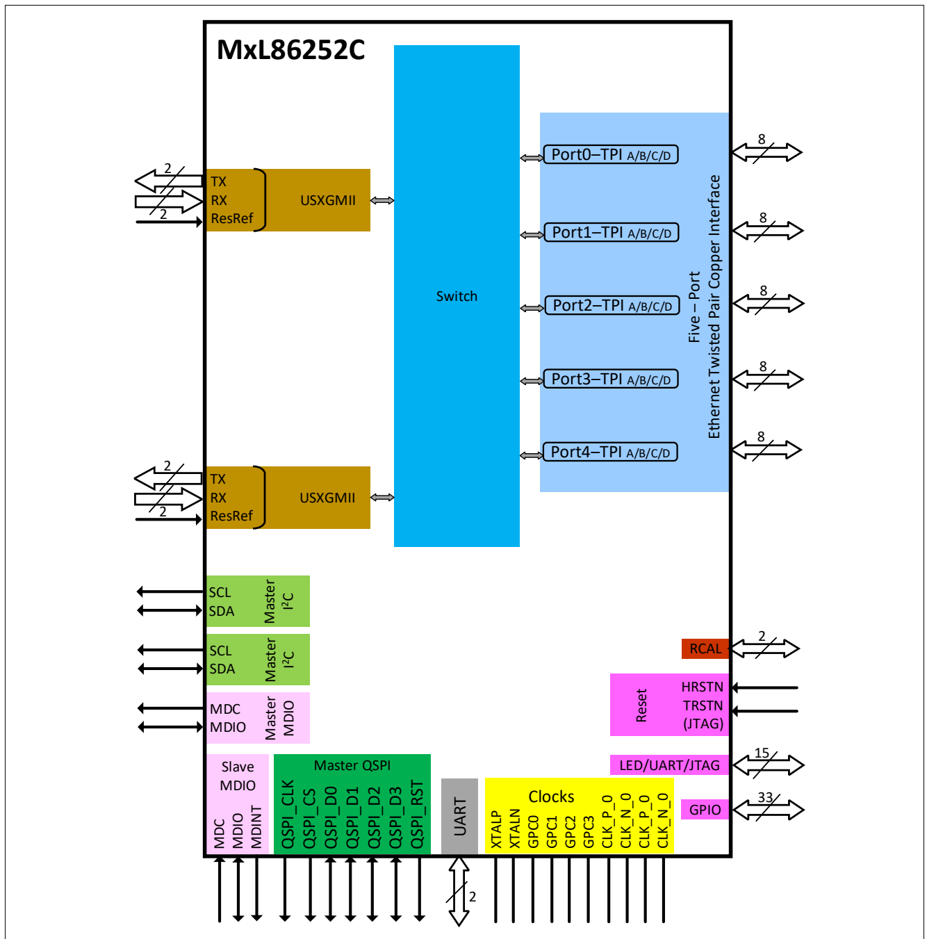
Figure 1 MxL86252C Block Diagram
