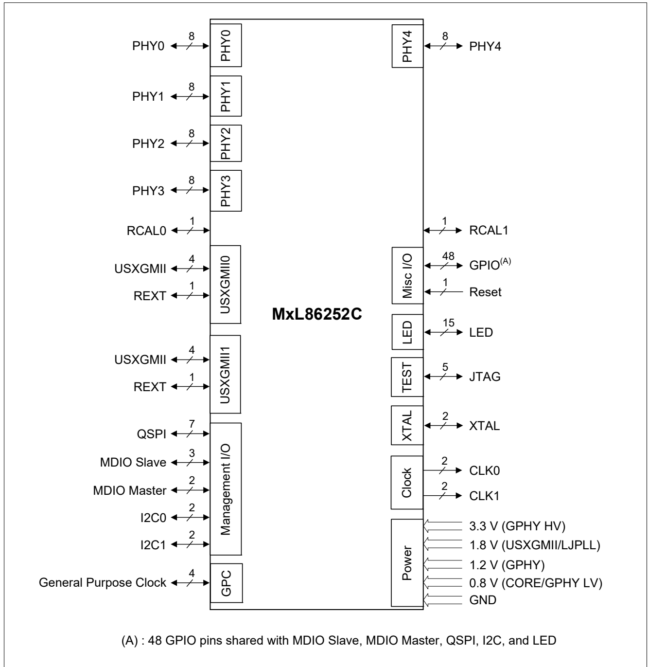
Figure 2 MxL86252C External Signal Overview
