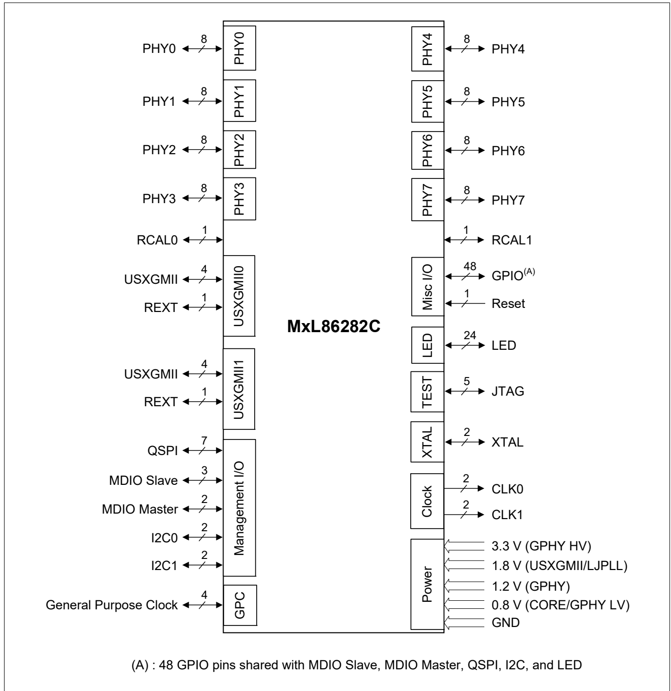
Figure 2 MxL86282C External Signal Overview
