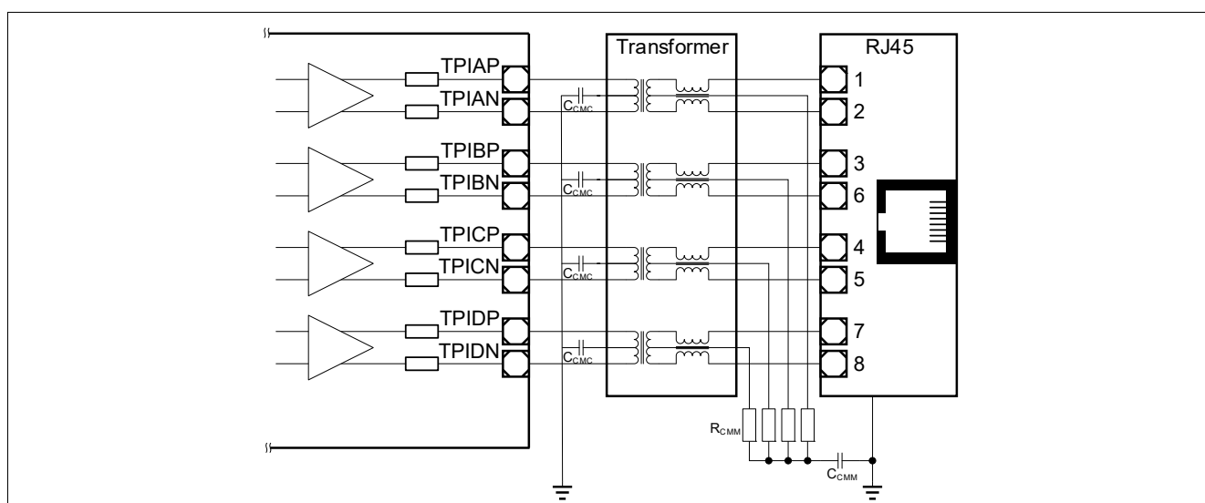
Figure 6 Twisted-Pair Interface of MxL86282C Including Transformer and RJ45 Plug
