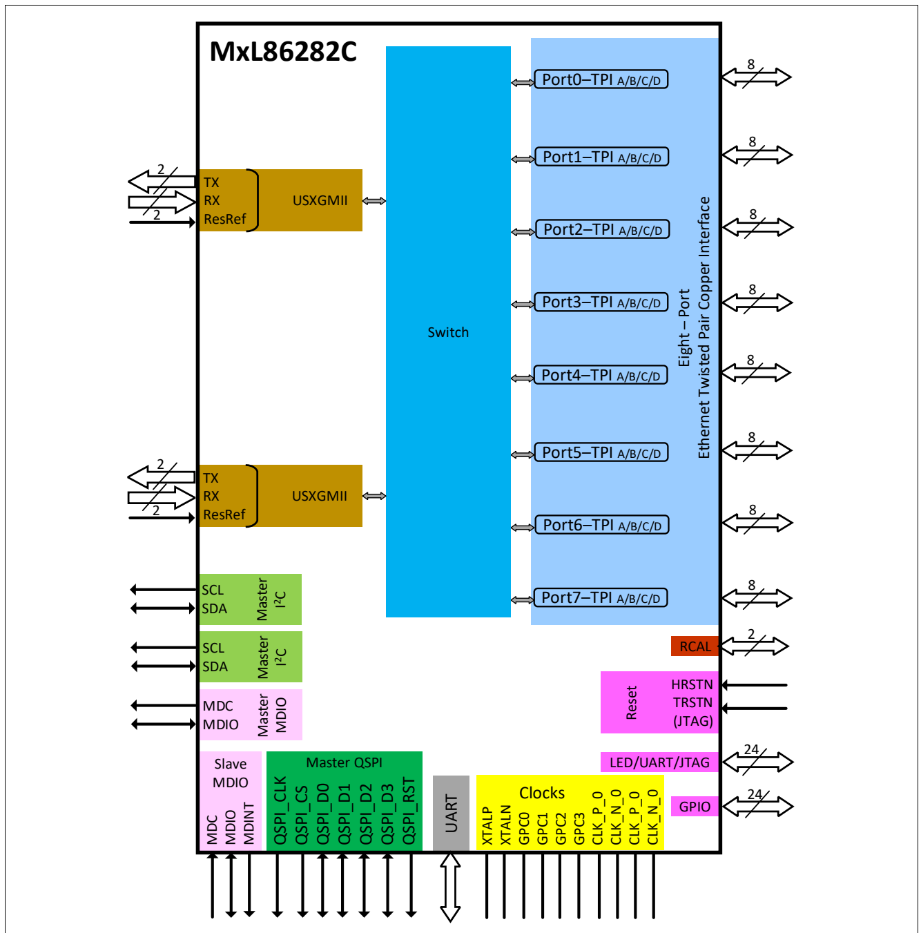
Figure 1 MxL86282C Block Diagram
