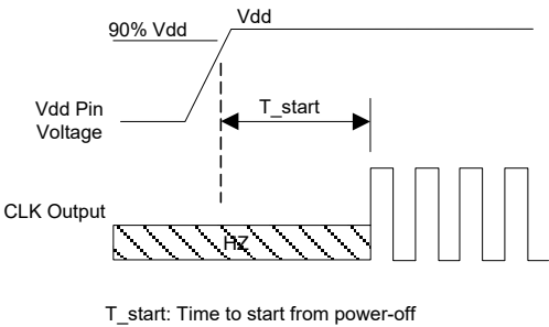
Figure 7. Startup Timing
