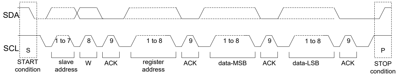
Figure 35. Parallel data byte format, write operation
