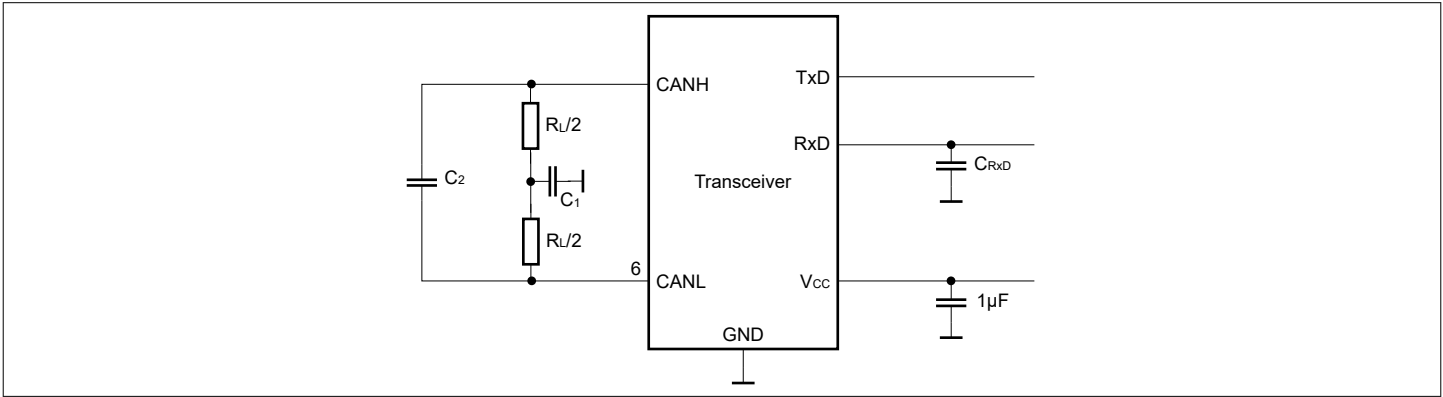
Figure 11 Test circuit
