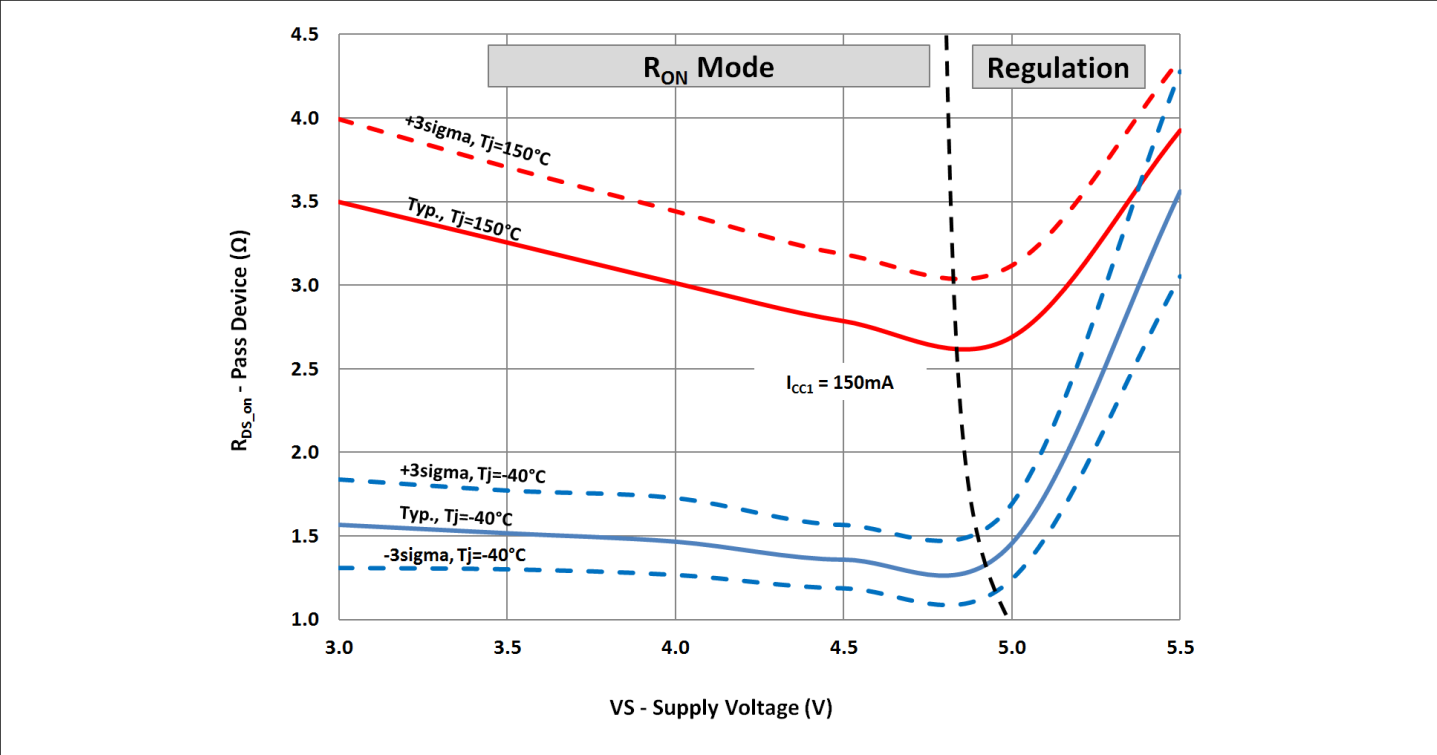
Figure 13 On-resistance range of VCC1 pass device during low drop operation for I_{CC1} = 150\text{mA}
