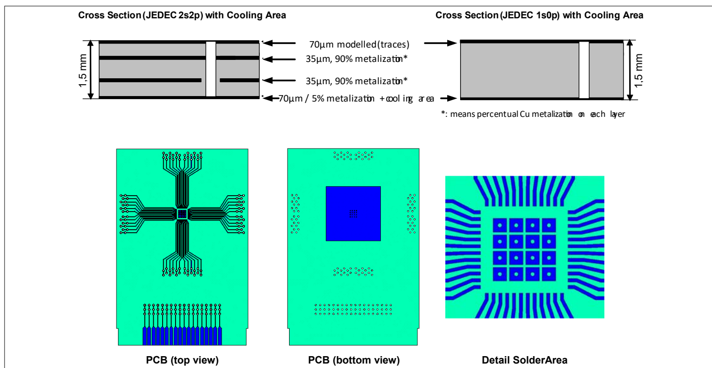
Figure 63 Board Setup
