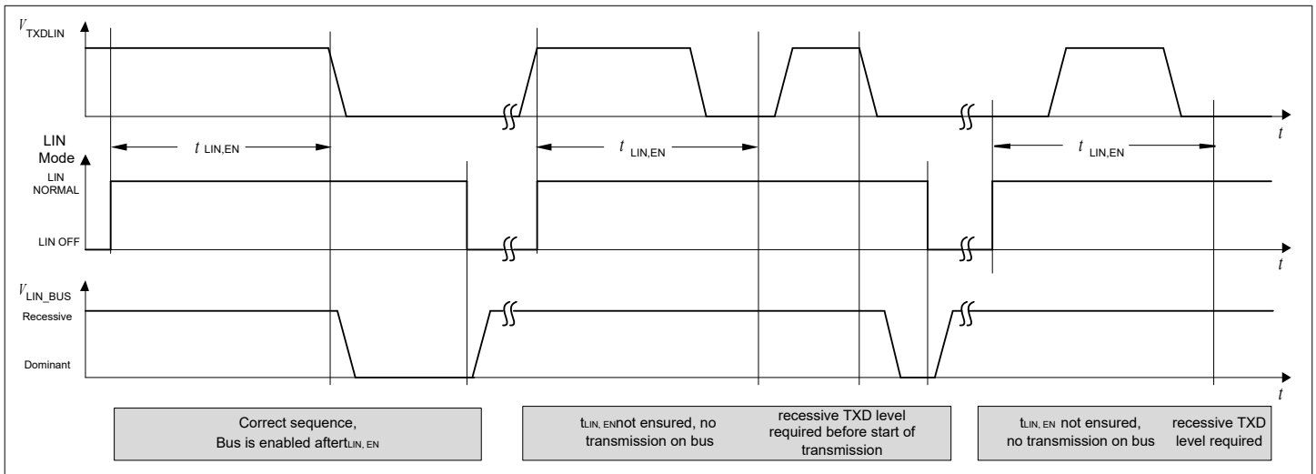
Figure 34 LIN Transceiver Enabling Sequence
