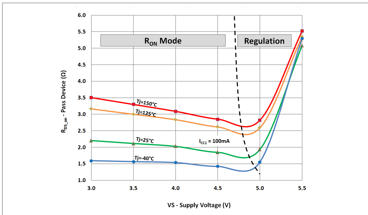
Figure 12 Typical on-resistance of VCC1 pass device during low drop operation for I_{CC1} = 100\text{ mA}
