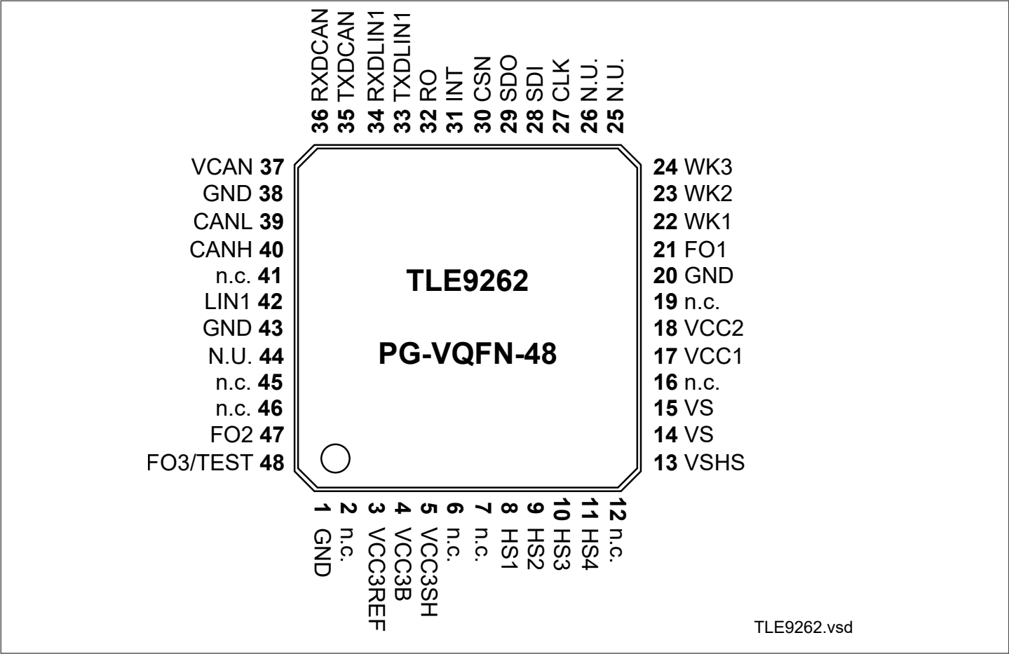
Figure 2 Pin Configuration
