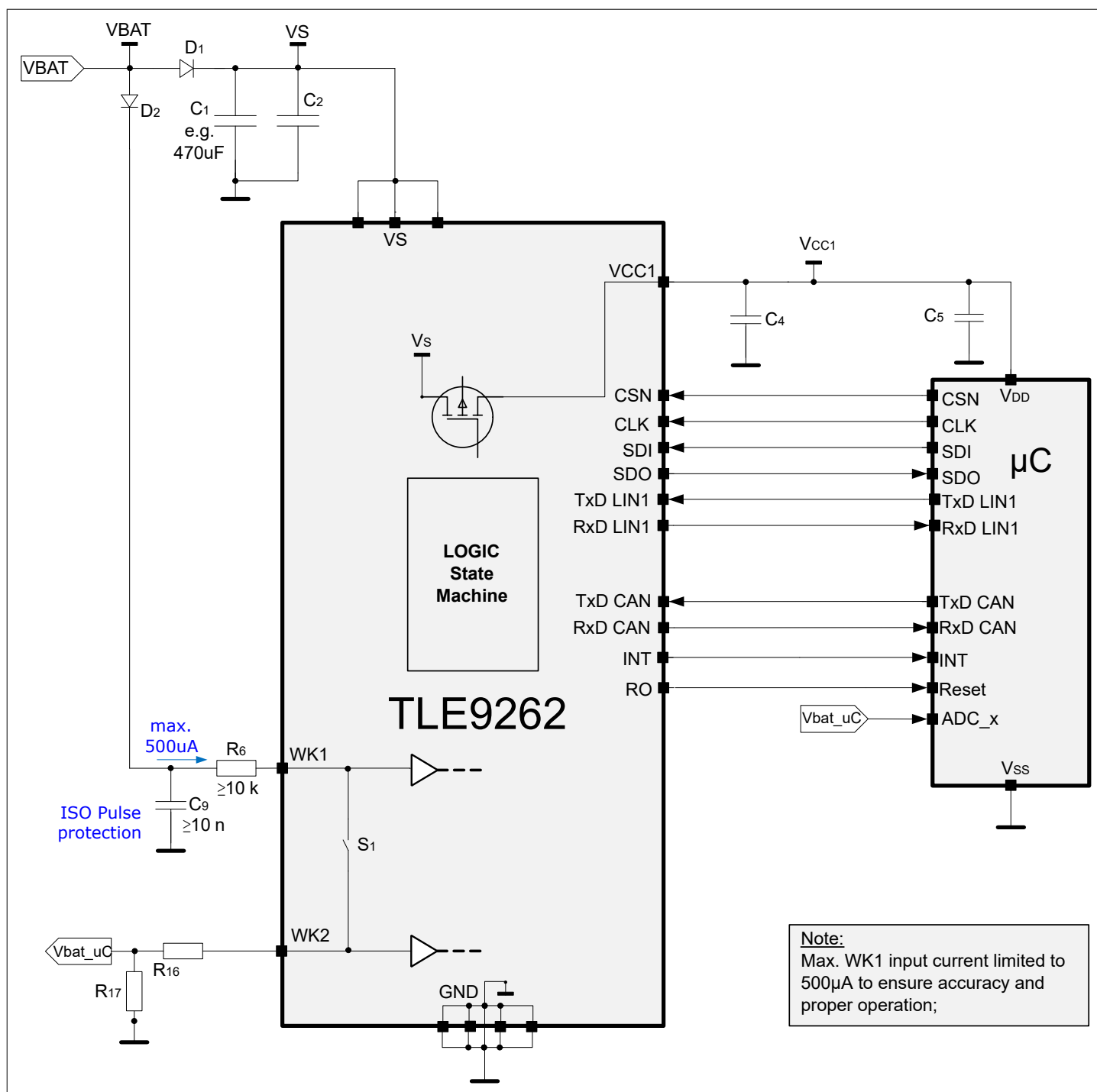
Figure 60 Simplified Application Diagram with the Alternate Measurement Function via WK1 and WK2
