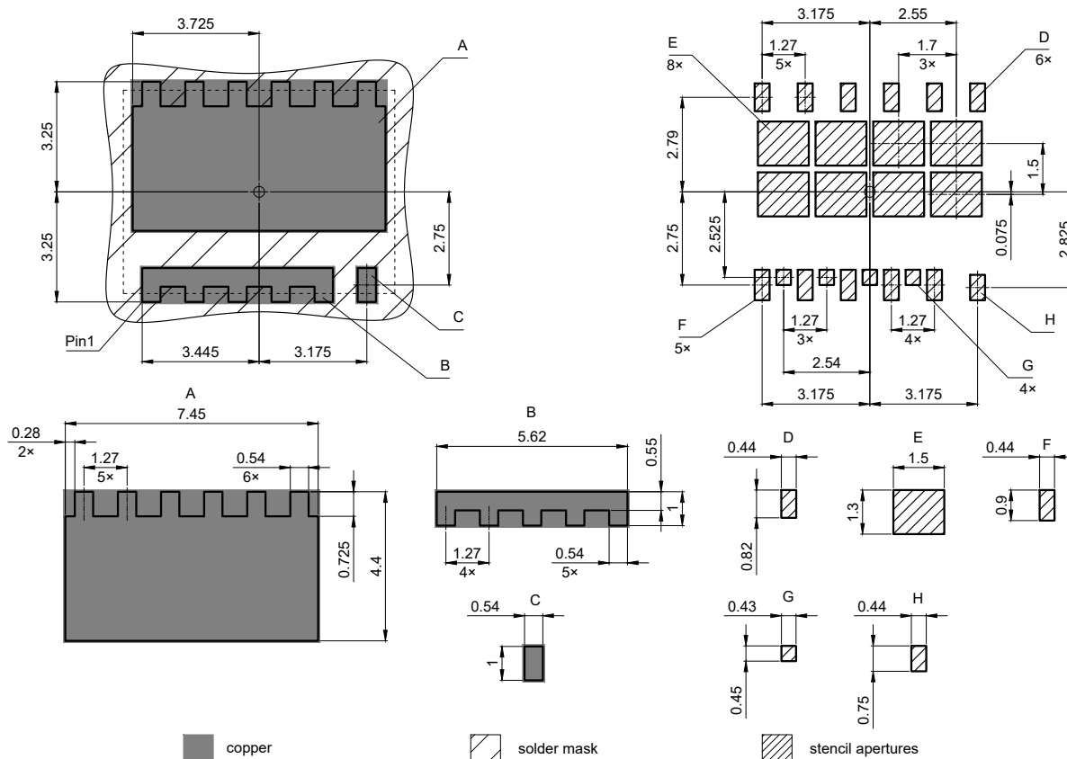
Figure 2 Outline Boardpad (PG-TSON-12), dimensions in mm
