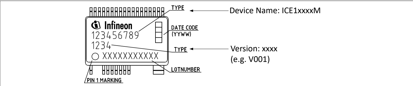
Figure 13 Marking PG-DSO-27-1
