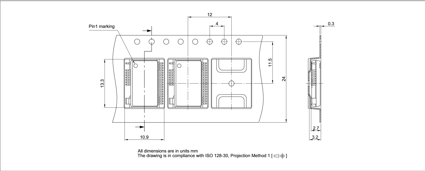
Figure 14 Packaging PG-DSO-27-1
