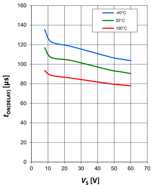
Typical performance characteristics (continued)
