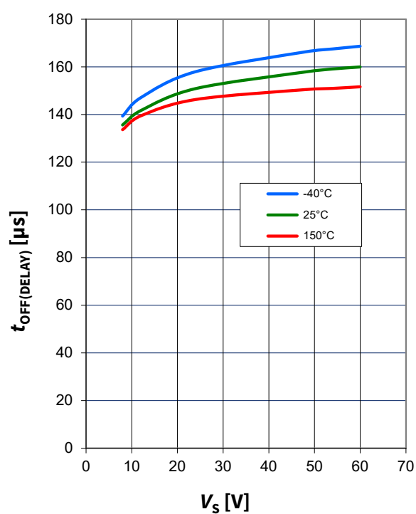
Turn off time
