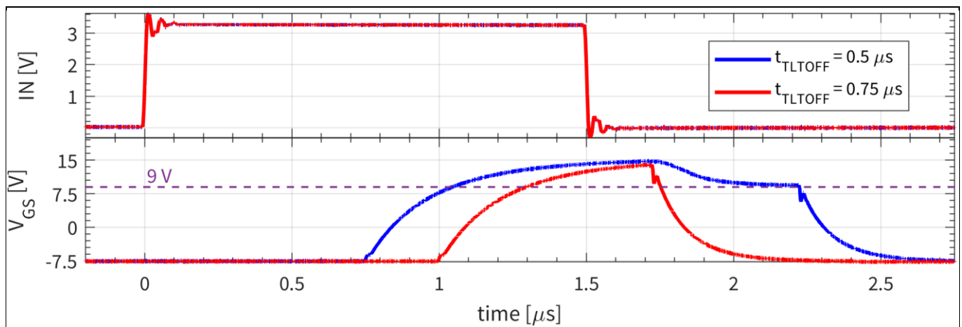
Figure 22 Two-level turn-off short on-pulse behavior; intermediate TLTOff voltage = 9 V, t_{\text{CLAMPfilter},x} = 370 \text{ ns}
