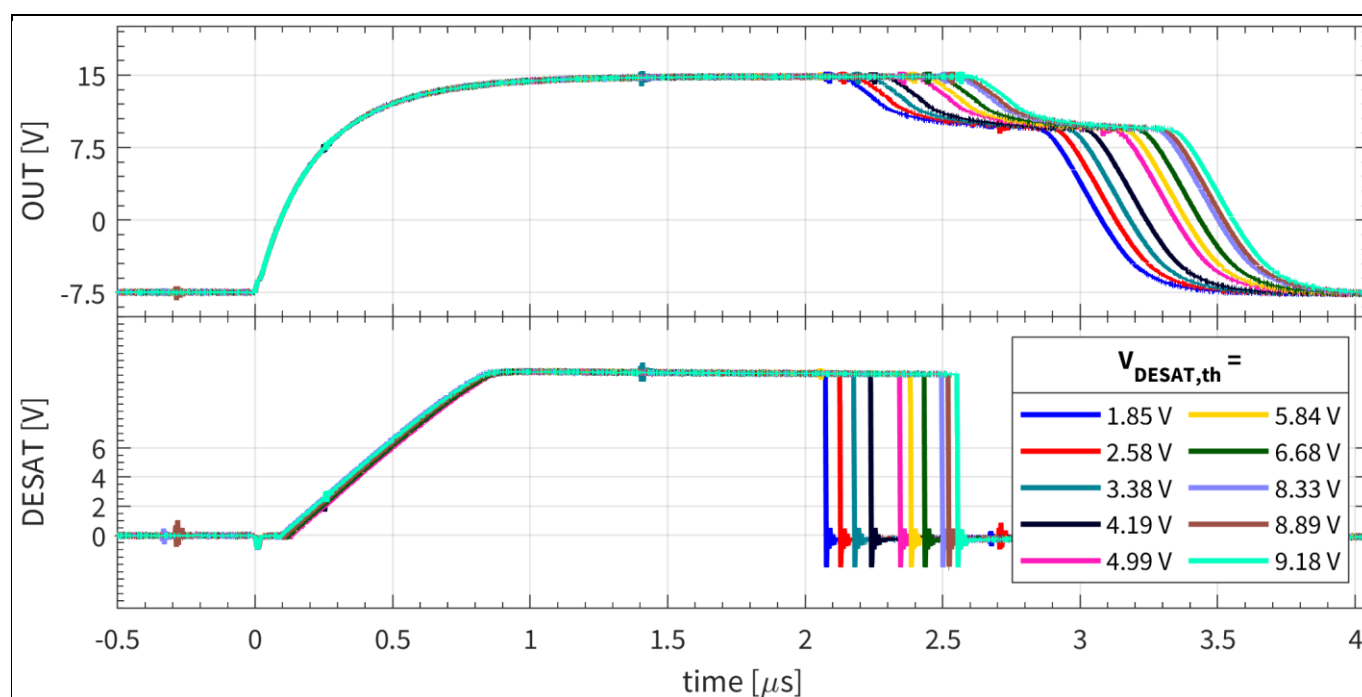
Figure 17 DESAT threshold voltage examples with LEB = 100 \text{ ns} and t_{DESAT} = 1575 \text{ ns}
