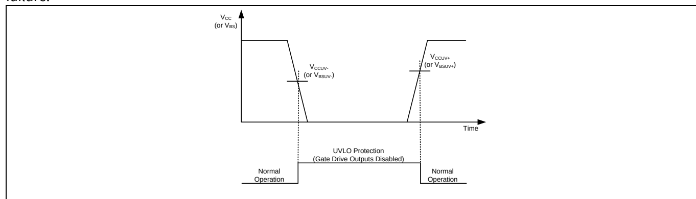
Figure 13 UVLO protection
