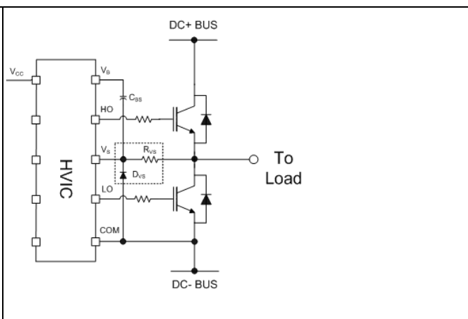
Figure 26 Clamping diode between COM and V_S
