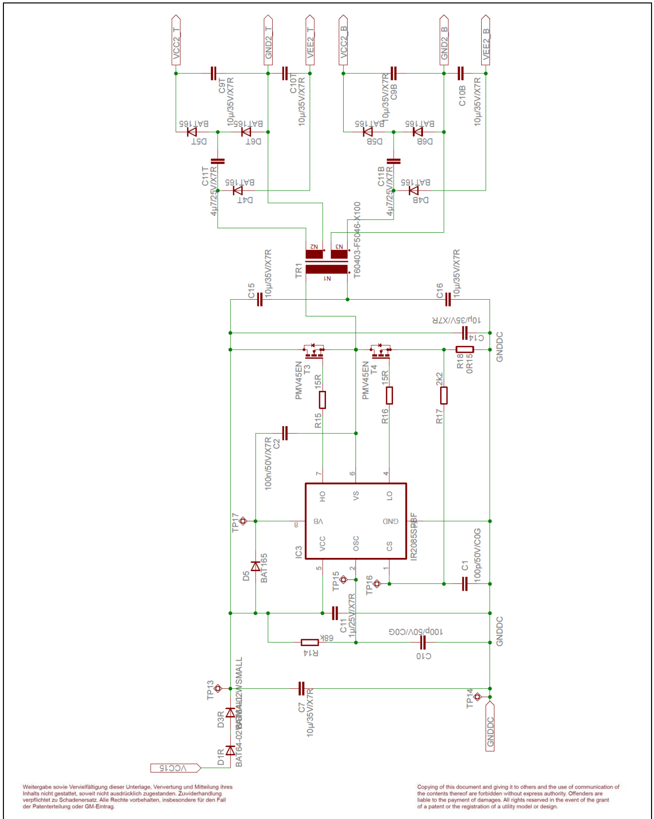
Figure 9 Schematic of isolated bipolar gate supply for high side and low side channel
