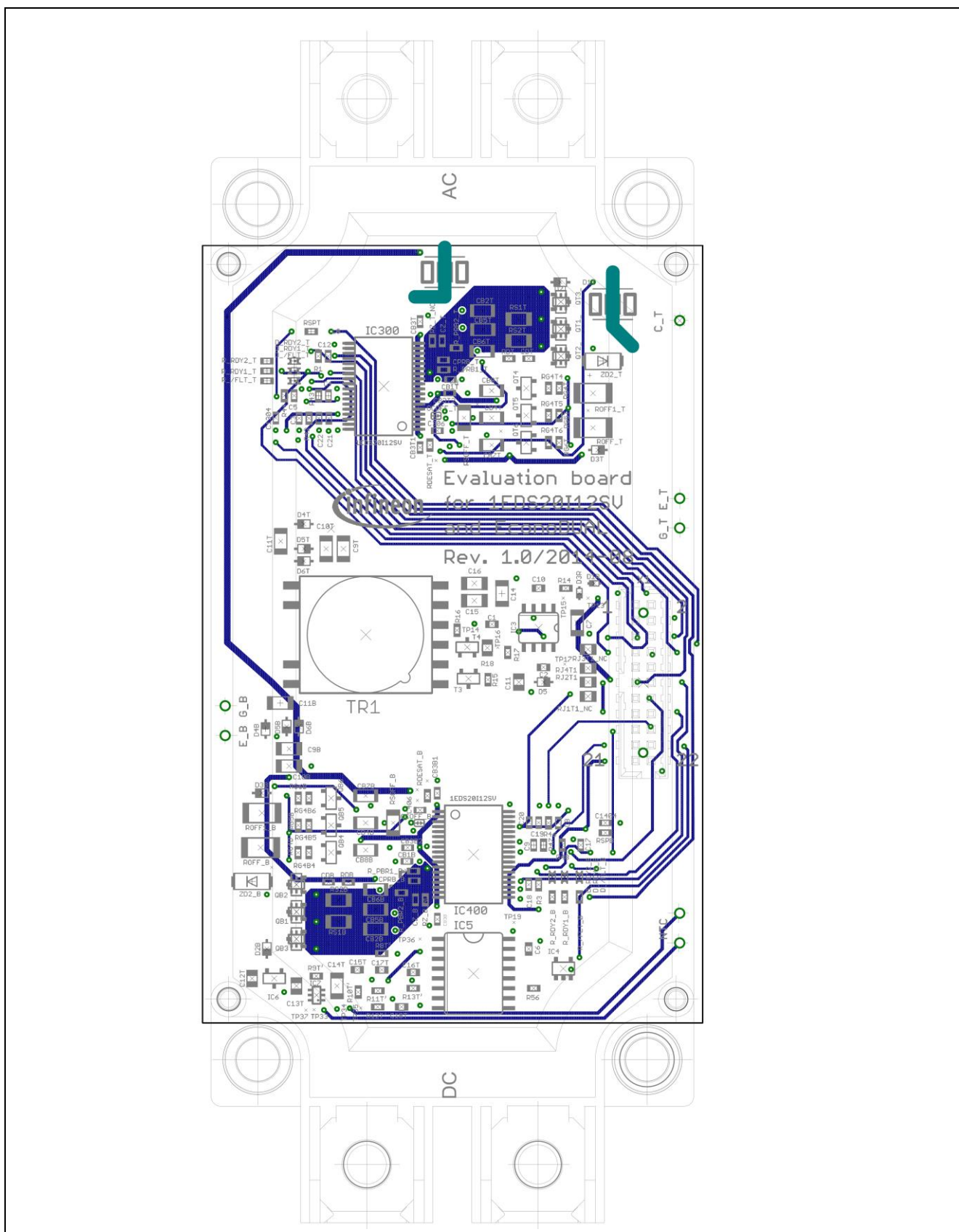
Figure 16 Inner layer 1
