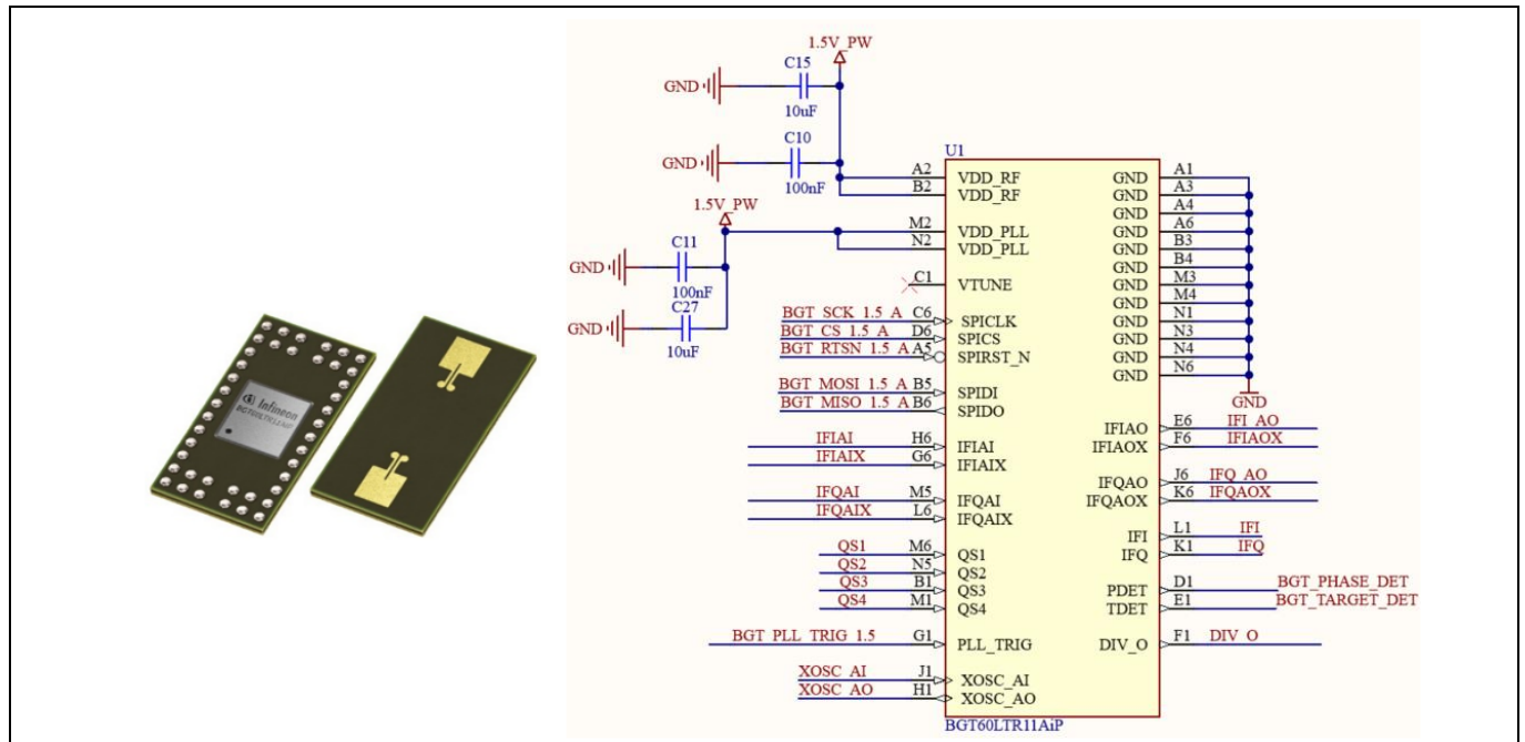
Figure 5 Package and pin-signal assignment of BGT60LTR11AIP MMIC
