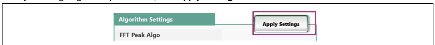
Figure 26 Apply settings
