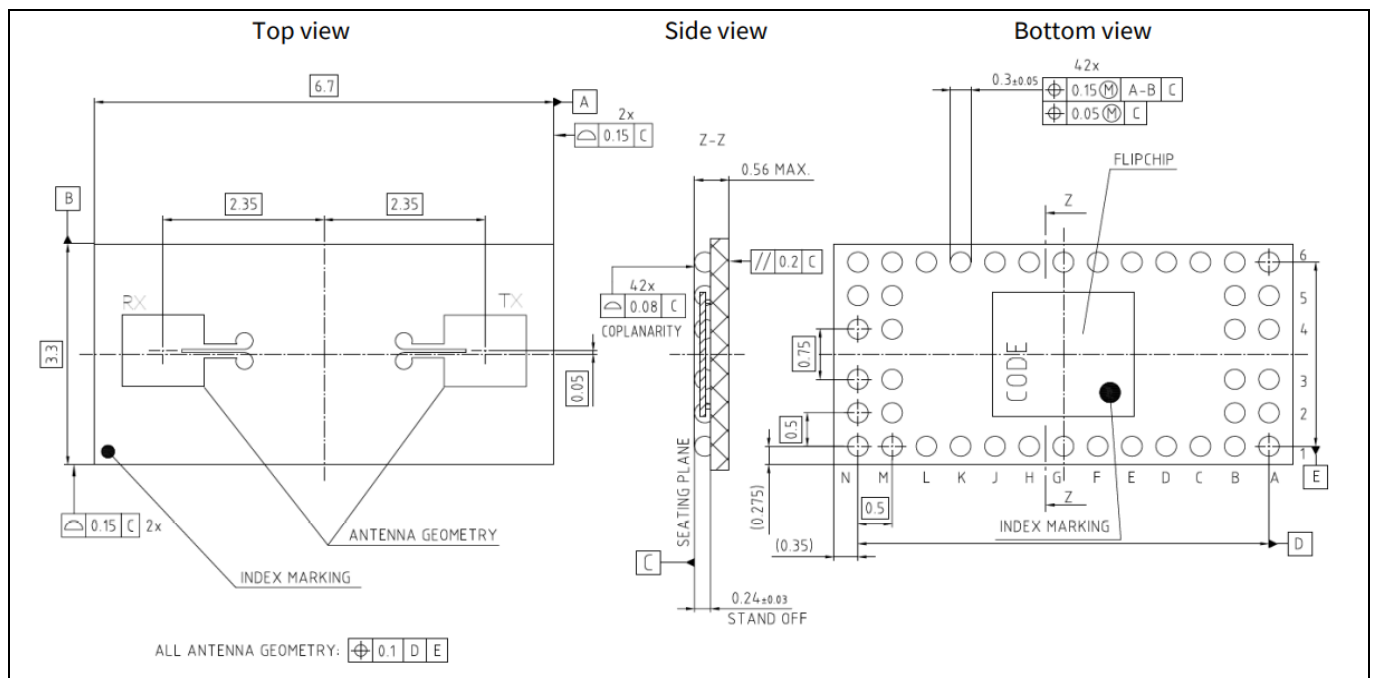
Figure 6 Top, side, and bottom views of BGT60LTR11AIP MMIC package (dimensions in mm)
