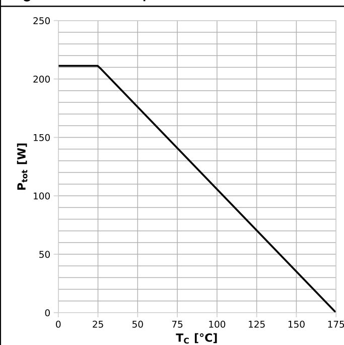
Diagram 1: Power dissipation
