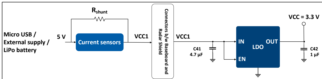
Figure 4 Block diagram – power supply concept
