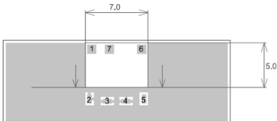
Top view of M20045-1 host PCB footprint
