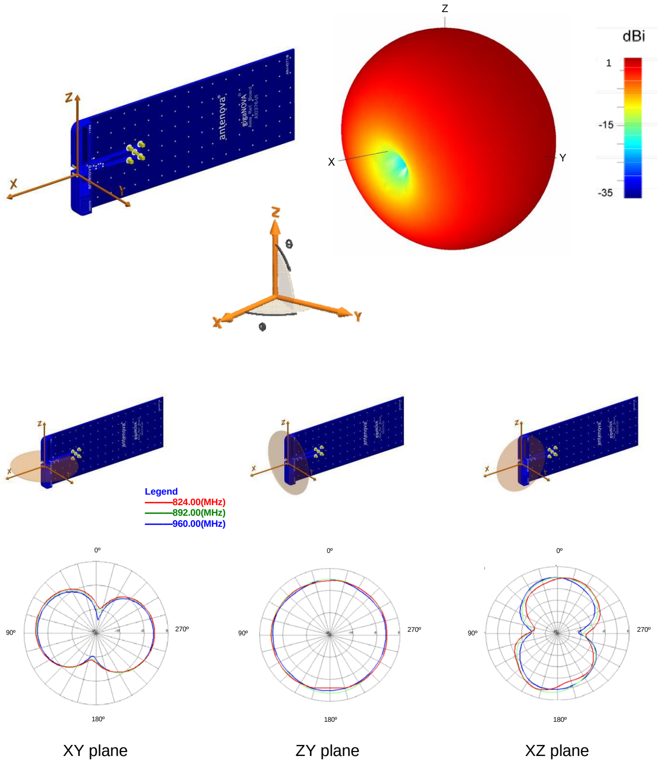
Patterns show combined polarisations measured on reference board A10376-U1. 3D Pattern measured at 890MHz
