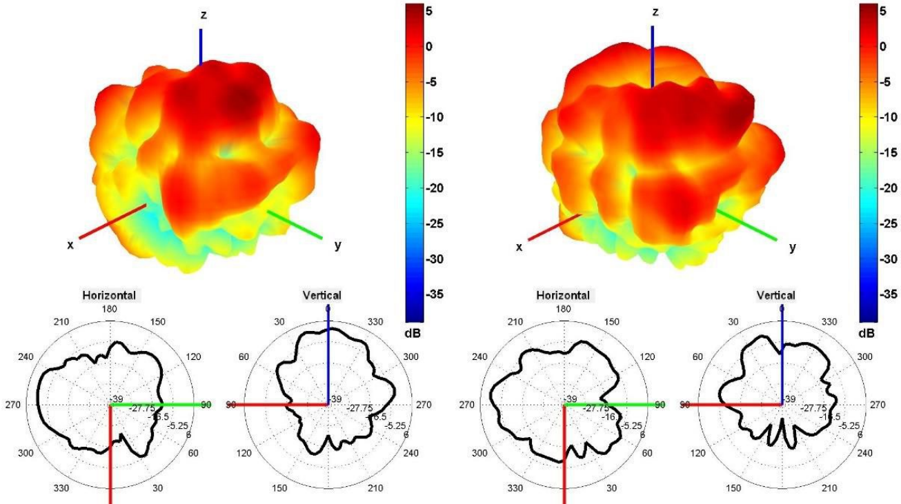
4500 and 5500 MHz Radiation pattern
