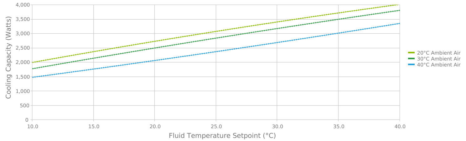
VRC2400-A1-20-BV2 Cooling Capacity - 60Hz 100% Water Flow = 17.4 L/min
