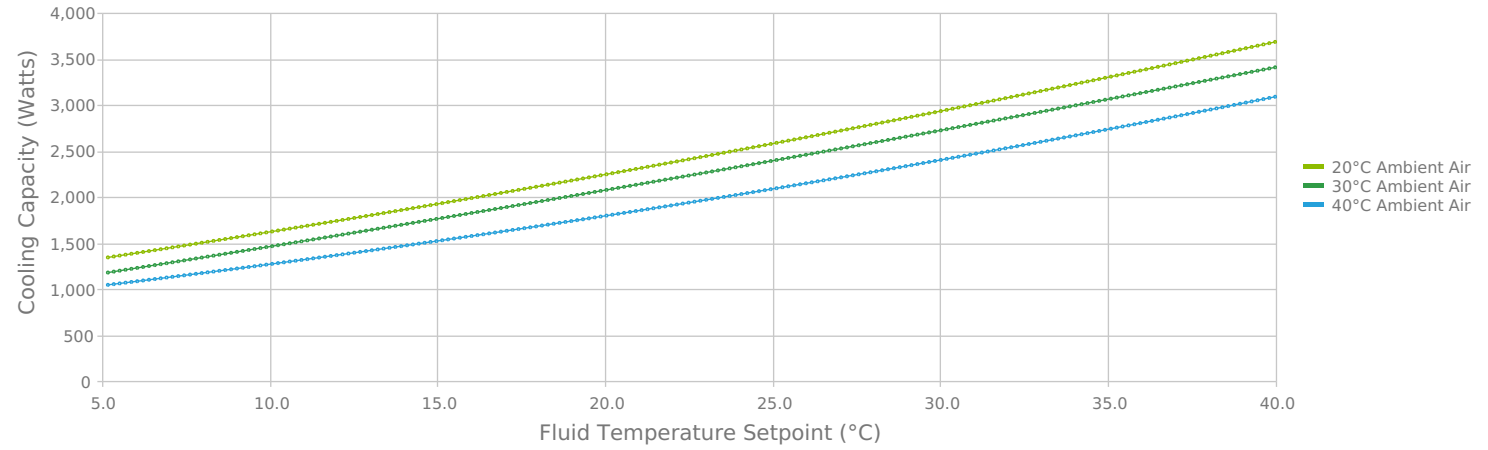
VRC2400-A1-20-BV2 Cooling Capacity - 50Hz 60/40 Water-Glycol Flow = 17.4 L/min
