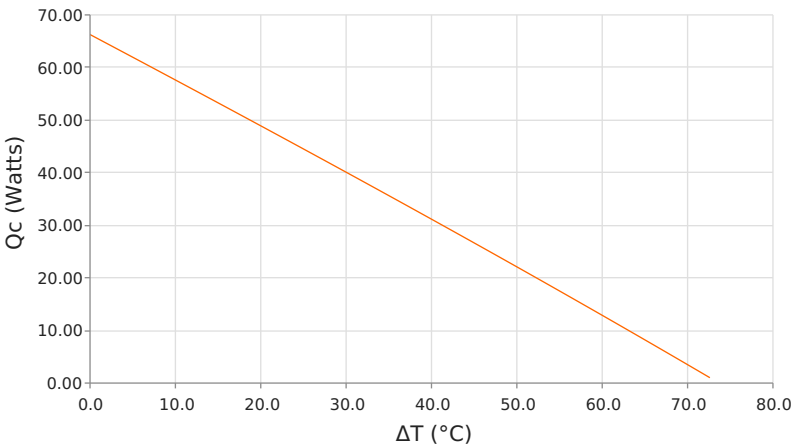
Heat Pumped at Cold Side ( Q_c ) T_{hot} = 35\text{ }^{\circ}\text{C} | operating = 6.7 Amps
