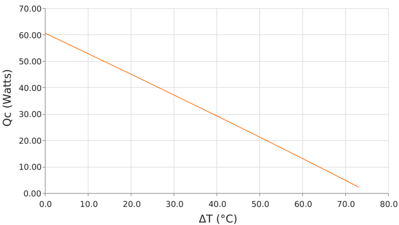
Heat Pumped at Cold Side ( Q_c ) T_{hot} = 50\text{ }^{\circ}\text{C} | operating = 6.1 Amps
