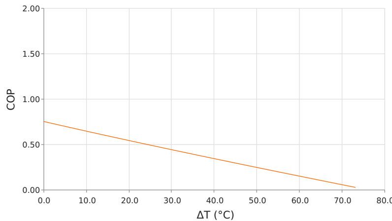
Coefficient of Performance ( COP = Q_c/P_{in} ) T_{hot} = 50\text{ }^{\circ}\text{C} | operating = 6.1 Amps
