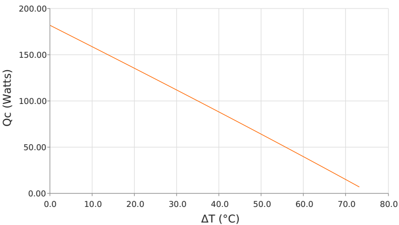
Heat Pumped at Cold Side ( Q_c ) T_{hot} = 50\text{ }^{\circ}\text{C} | operating = 18.4 Amps
