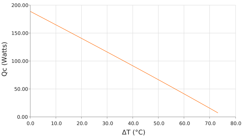
Heat Pumped at Cold Side ( Q_c ) T_{hot} = 50\text{ }^{\circ}\text{C} | operating = 12.2 Amps
