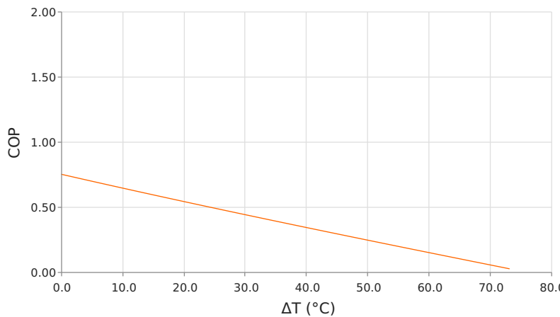
Coefficient of Performance (COP = Q_c/P_{in} ) T_{hot} = 50\text{ }^{\circ}\text{C} | operating = 12.2 Amps
