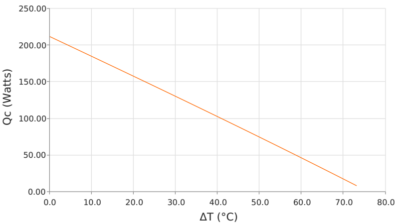
Heat Pumped at Cold Side ( Q_c ) T_{hot} = 50\text{ }^{\circ}\text{C} | operating = 11.3 Amps
