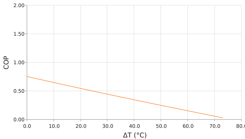
Coefficient of Performance (COP = Q_c/P_{in} ) T_{hot} = 50\text{ }^{\circ}\text{C} | operating = 11.3 Amps
